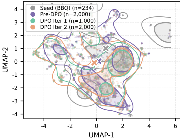
(b) Qwen2.5-VL-7B — UMAP
