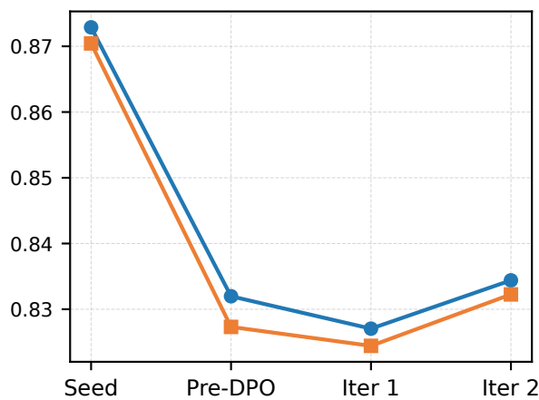
Centroid Distance
