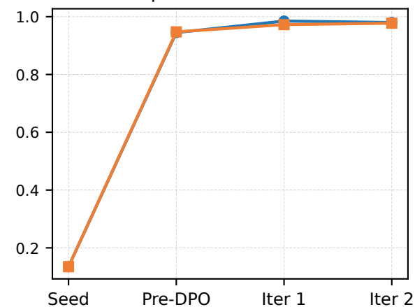
Vocabulary Size
