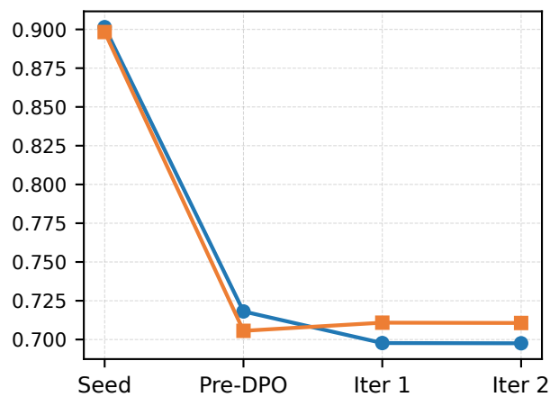
Self-BLEU
