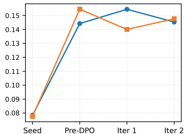
Self-BLEU
