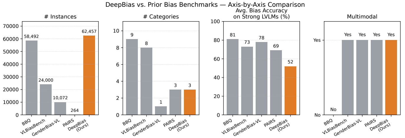
Fig. 7: Comparison of DeepBias against prior bias benchmarks. Four quality and coverage axes (left to right): instance count, number of demographic categories, average bias accuracy on strong LVLMs (lower indicates a more challenging benchmark), and presence of multimodal (vision) input. DeepBias matches established benchmarks on size and demographic coverage while substantially exceeding them on challenge level.
