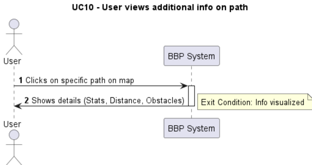
Figure 10: Use Case Diagram for UC10: User views additional information about selected path on map
