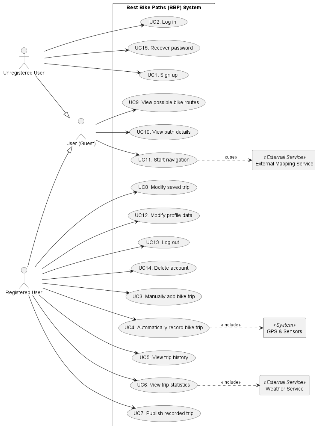
Figure 1: High level Use Case Diagram
