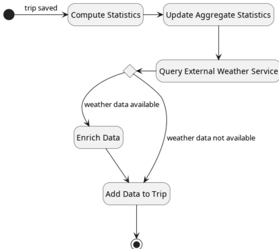
Figure 5: Statistics Generation State Diagram
