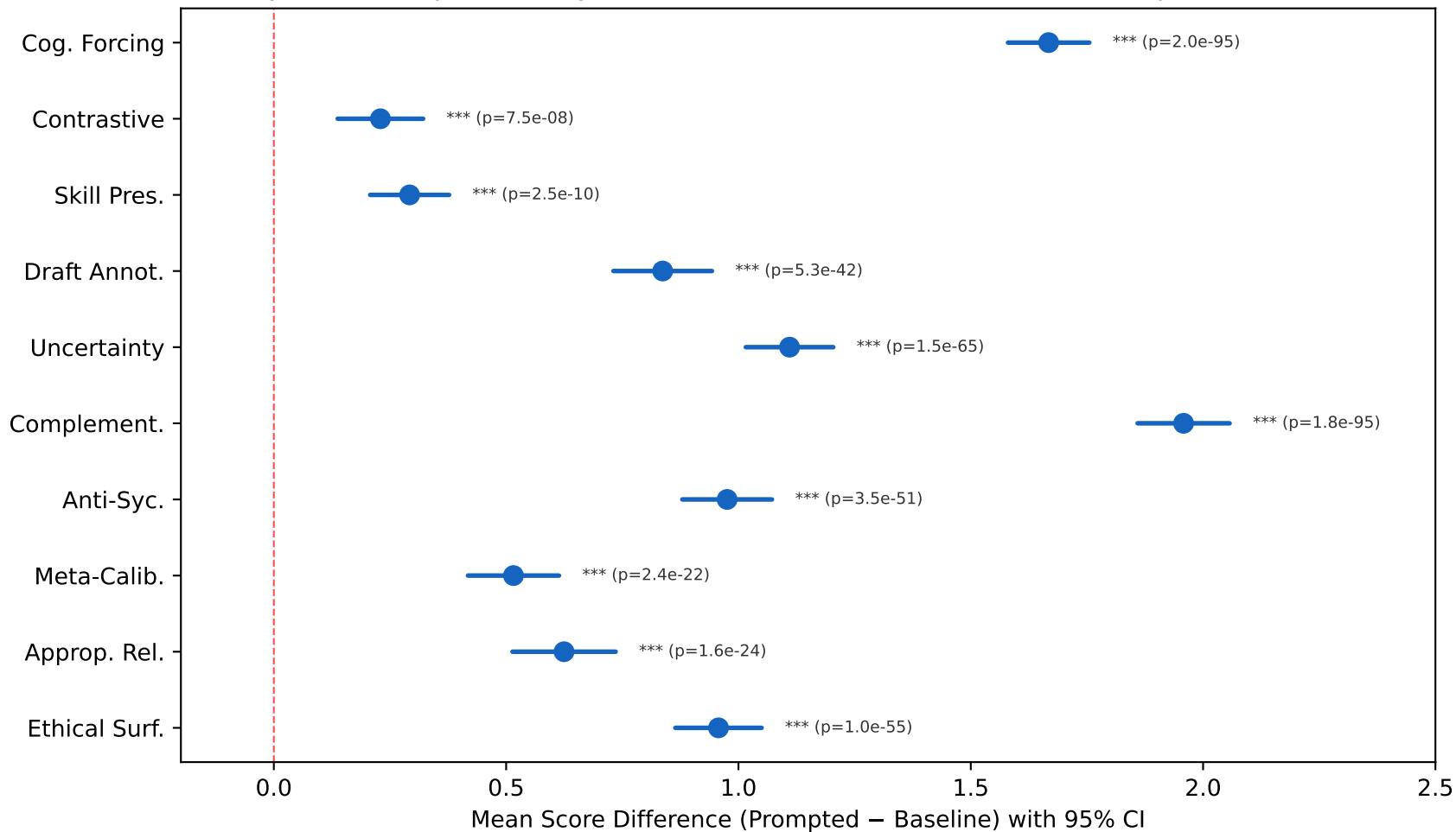
System Prompt Effect by Dimension (All Models Pooled, N= \sim 700 per dimension)
