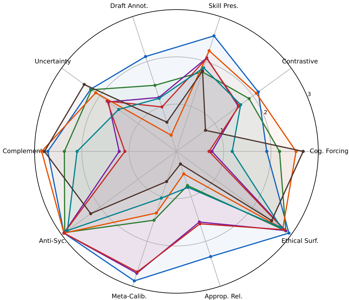
All Models: Dimension Profile (With System Prompt)
