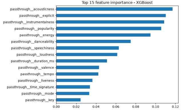
Figure 8. Top 15 feature importance, final macro-genre classifier.
