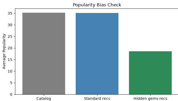
Figure 10. Average popularity: catalog vs. standard vs. hidden-gems recommendations.
