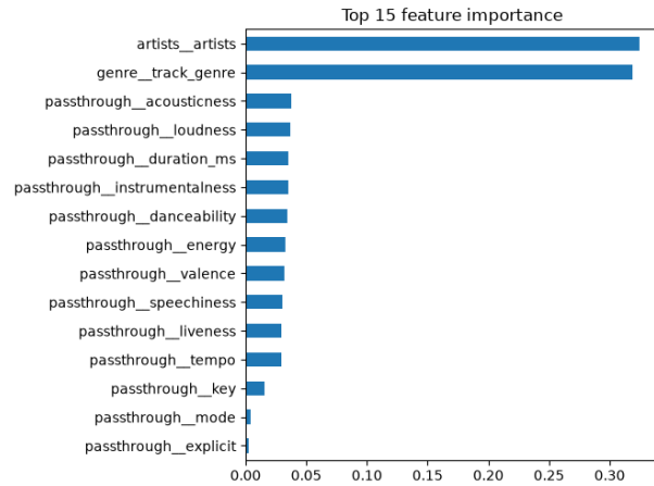
Figure 4. Top 15 feature importance, final Random Forest model.
