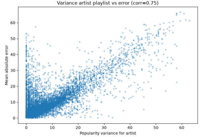
Figure 5. Artist catalog popularity variance vs. mean absolute prediction error.
