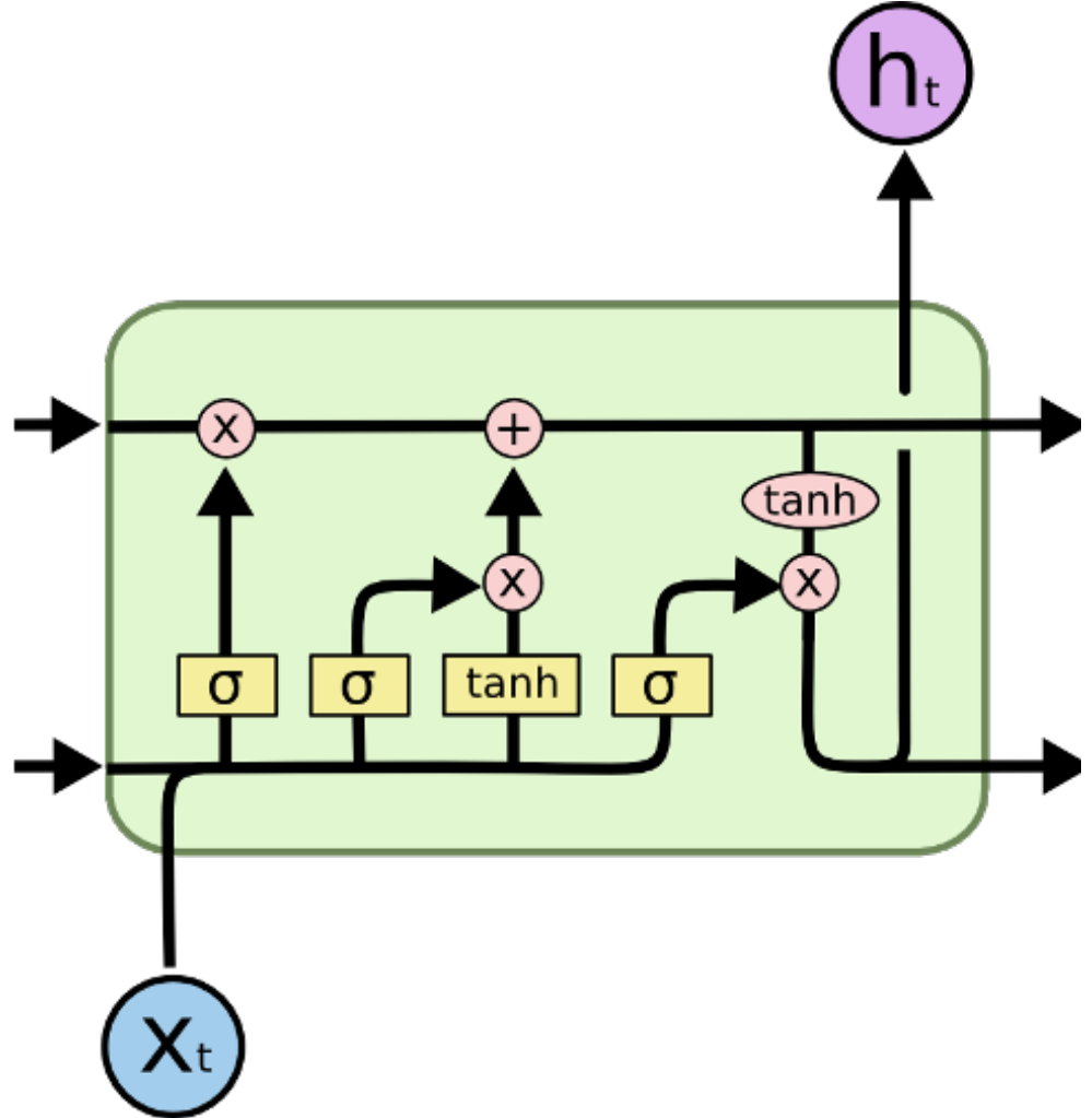
LSTM
