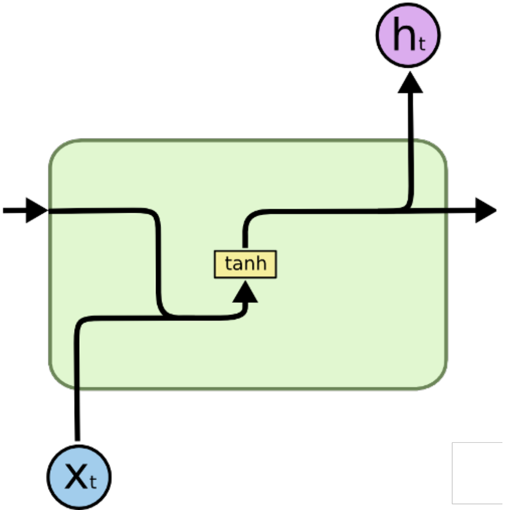
Simple RNN
