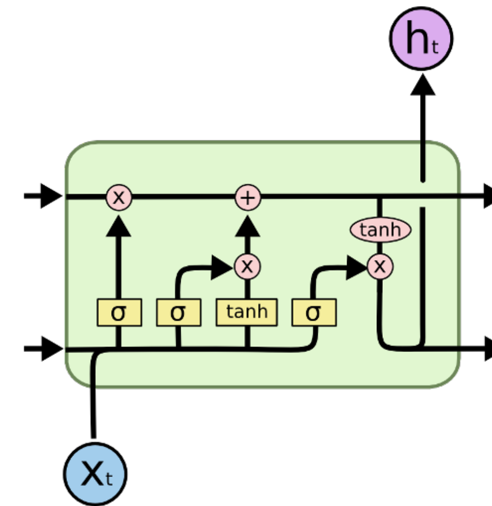
LSTM
