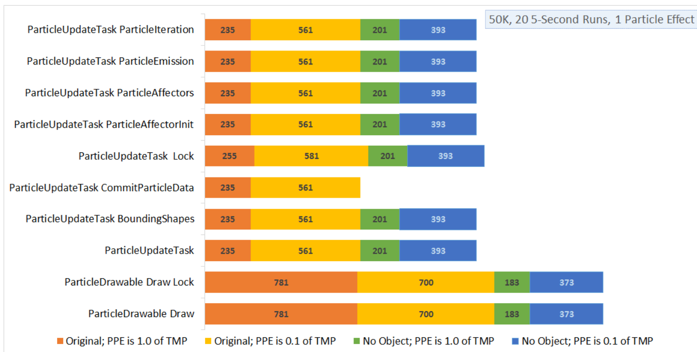
Figure 5.5 A graph showing the number of section calls for various sections of code for a single particle effect. This most notably shows that the section calls for the Original data series had significantly higher values in the drawing functions than the ones in the No Object data series.
