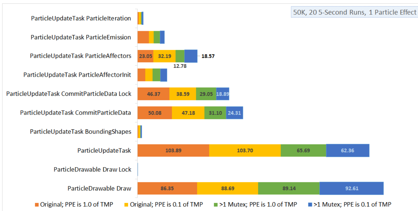
Figure 4.7 A graph showing the time spent in various sections of code for a single particle effect. Note that the "ParticleUpdateTask CommitParticleData Lock" section is timing the particle array lock for the > 1 Mutex data series. The > 1 Mutex data series shows improvement in the CommitParticleData function from the Original. For 0.1 TMP, CommitParticleData went down from 47 seconds to 24. For 1.0 TMP, CommitParticleData went down from 50 seconds to 31. This was approximately a 40% increase in speed.
