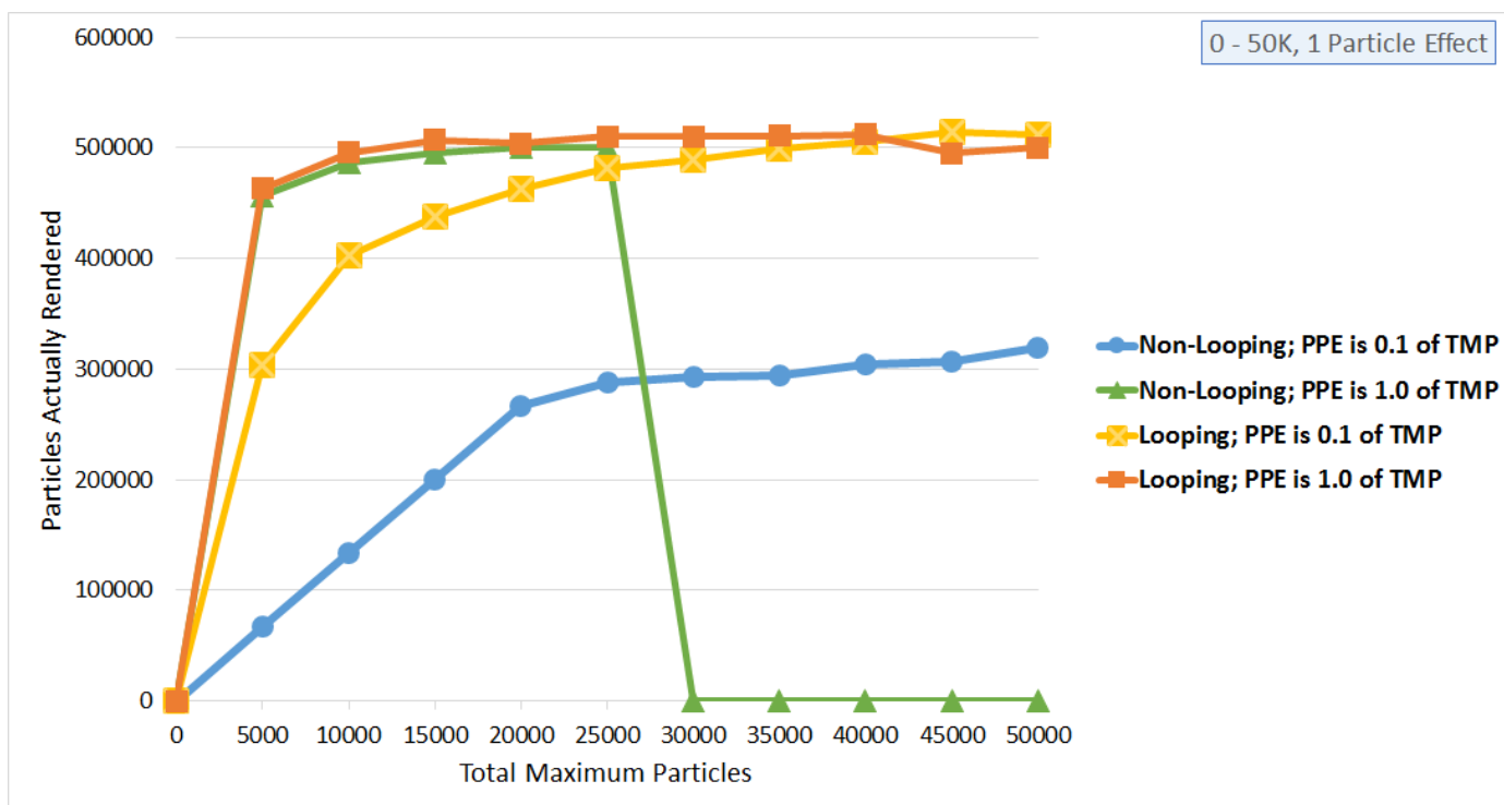
Figure 5.19 A graph showing particles actually rendered over total maximum particles for a single particle effect. As mentioned in Figure 5.18, this graph illustrates that the Non-Looping data series, overall, does not render as many particles as the Looping data series. At 30,000 TMP, the Non-Looping data series does not render any particles at all.
