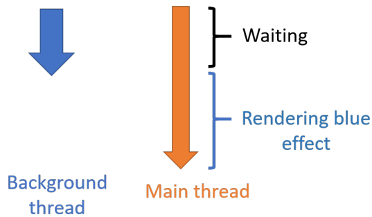
Figure 4.23 The lifetime of a single particle effect in relation to its scheduled background thread and the main thread.
