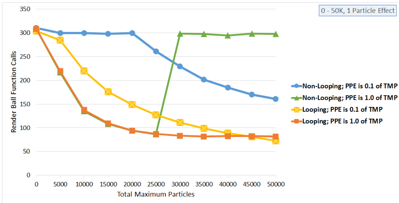
Figure 5.18 A graph showing render ball function calls over total maximum particles for a single particle effect. This shows that, overall, the Non-Looping data series performs better (or renders more particles) than the Looping (i.e. Original) data series. However, it is important to pair this fact with two other observations: (1) Figure 5.19 shows that the Non-Looping data series renders considerably less particles, and (2) at about 30,000 TMP there is spike in render ball function calls .
