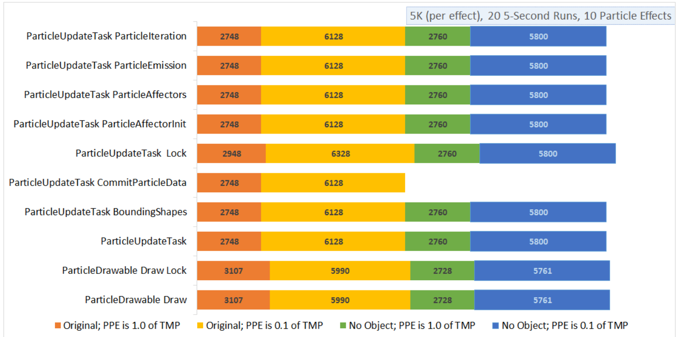
Figure 5.7 A graph showing the number of section calls for various sections of code for ten particle effects. This shows that removing the ConcurrentParticleData object for many particles did not affect the number of section calls; the Original and No Object data series both have similar values for the multiple-burst (0.1 TMP) and single-burst (1.0 TMP) games.
