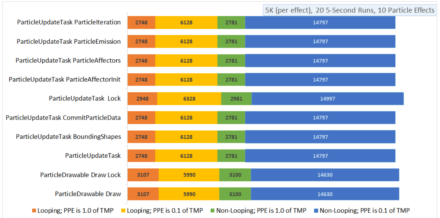
Figure 5.24 A graph showing the number of section calls for various sections of code for ten particle effects. This shows that: (1) The Non-Looping data series in multiple-burst (or 0.1 TMP) games have a significantly higher section call count than the Looping data series, and (2) The Non-Looping data series in single-burst (or 1.0 TMP) games approximately have the same section call counts as the Looping data series.
