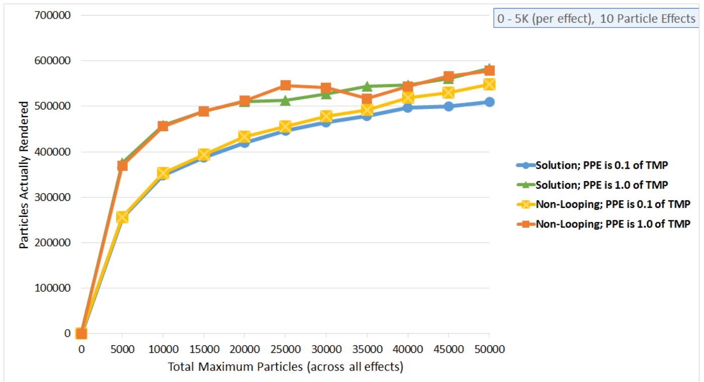
Figure 5.29 A graph showing particles actually rendered over total maximum particles for ten particle effects. Similar to Figure 5.28, this shows that the Solution and Non-Looping data series render about the same number of particles.
