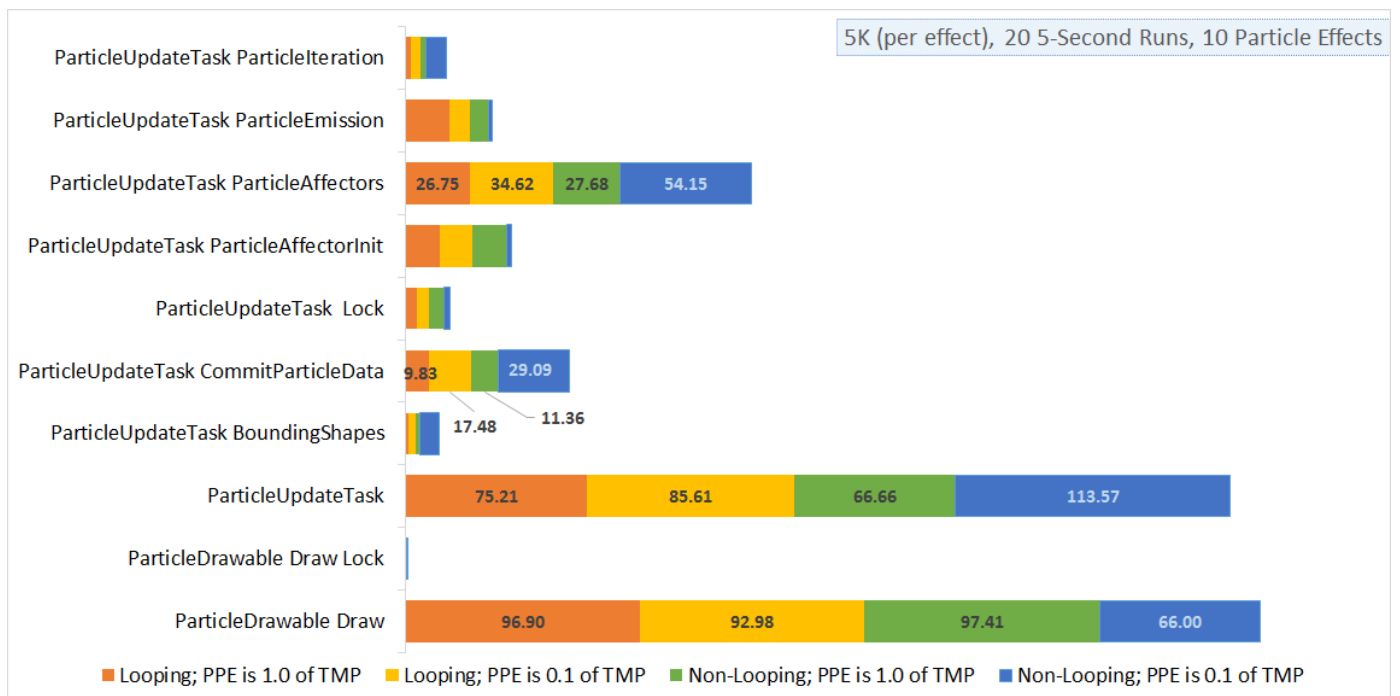
Figure 5.25 A graph showing the time spent in various sections of code for ten particle effects. This shows that: (1) The Non-Looping data series in multiple-burst (or 0.1 TMP) games have a higher run time for particle update functions and a lower run time for particle draw functions, and (2) The Non-Looping data series in single-burst (or 1.0 TMP) games have similar run times as the Looping data series.
