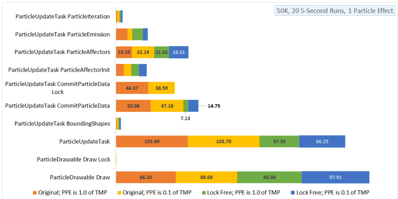
Figure 4.11 A graph showing the time spent in various sections of code for a single particle effect. CommitParticleData for the Lock Free data series, as expected, experienced a performance boost. For 0.1 TMP, the function went down from 47 seconds to 15. For 1.0 TMP, it went down from 50 seconds to 7. This was, respectively, about an 68% and 86% increase in performance.
