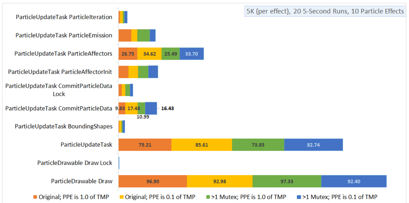
Figure 4.16 A graph showing the time spent in various sections of code for ten particle effects. Unlike in the single particle effect results, this shows not only no significant improvement to the CommitParticleData function, but it also shows that there was little contention to begin with in the Original data series.
