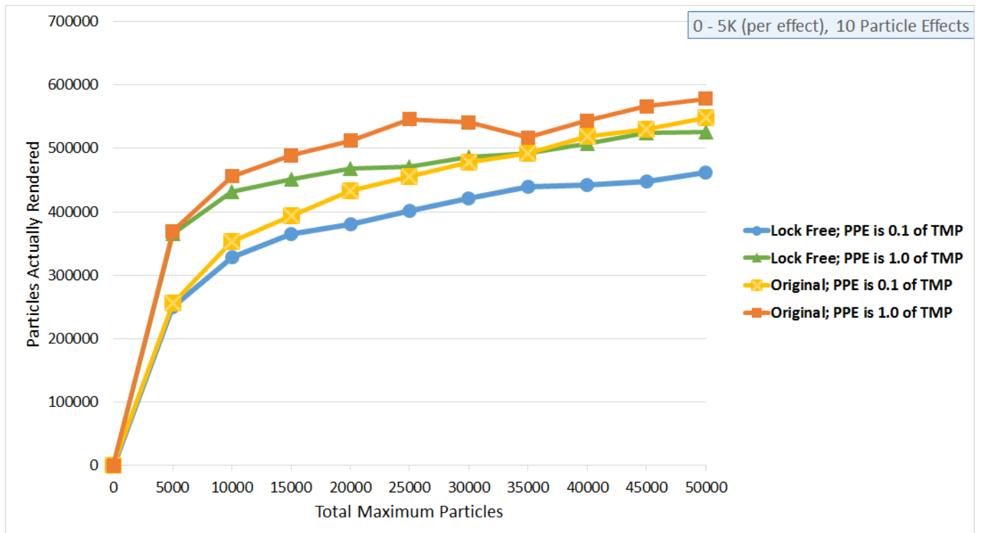
Figure 4.18 A graph showing particles actually rendered over total maximum particles for ten particle effects. Similar to the single particle effect results, the multiple-burst and single-burst (0.1 and 1.0 TMP, respectively) scenarios for the Lock Free data series are lower than the ones for the Original data series.
