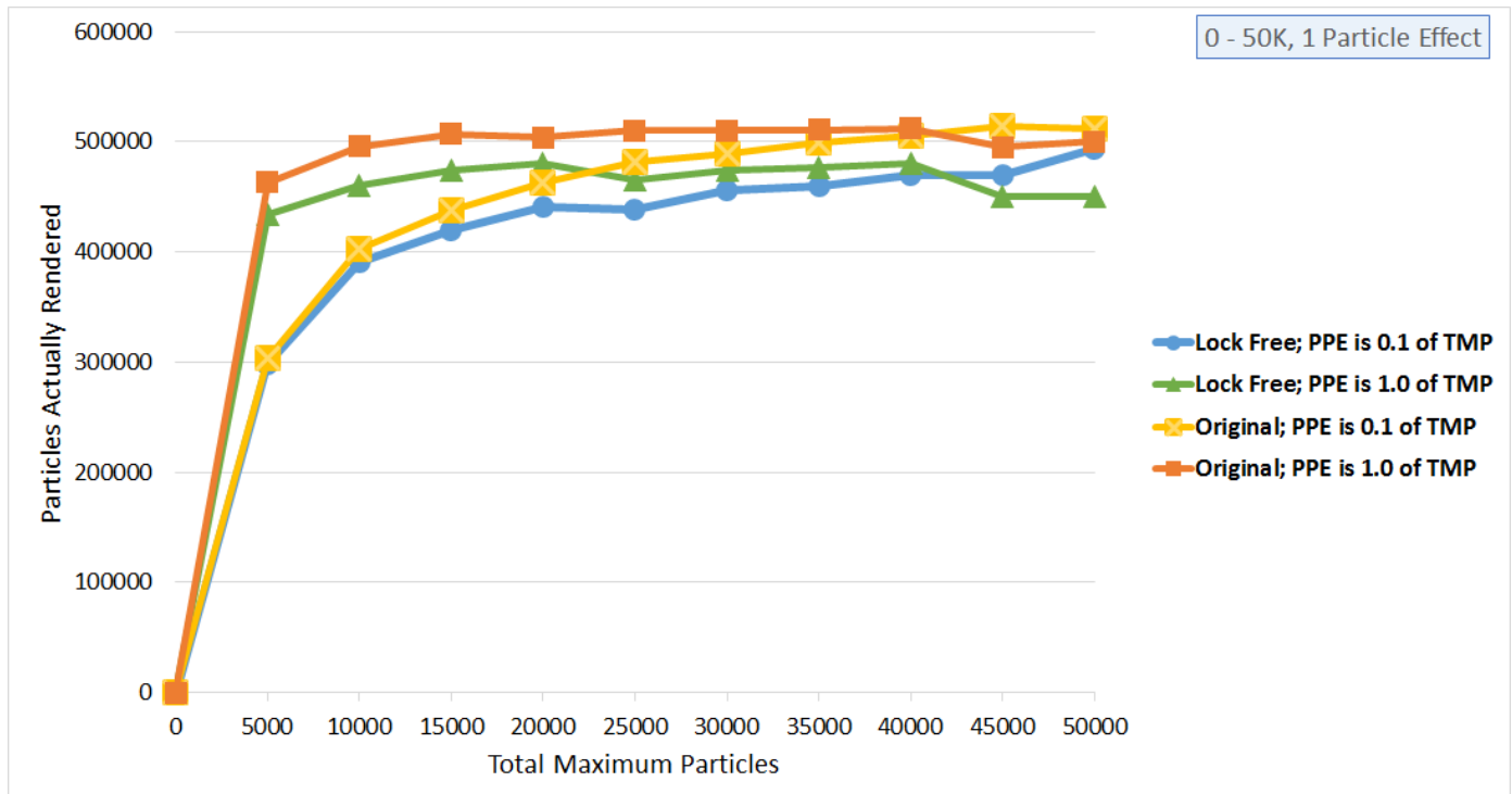
Figure 4.9 A graph showing particles actually rendered over total maximum particles for a single particle effect. This shows that changing Concurrent Particle Data to use a lock free data structure does not positively impact the number of times that particles are rendered. The multiple-burst and single-burst (0.1 and 1.0 TMP, respectively) scenarios for the Lock Free data series are lower (which means worse performance) than the ones for the Original data series.
