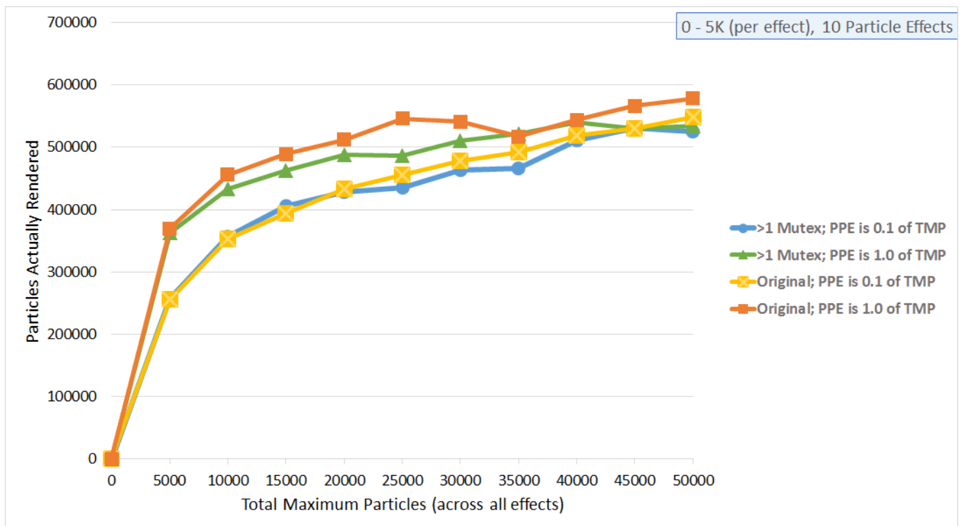
Figure 4.14 A graph showing particles actually rendered over total maximum particles for ten particle effects. The two data series, > 1 Mutex and Original, show no stark differences; their particles actually rendered values are nearly the same for the multiple-burst (0.1 TMP) and single-burst (1.0 TMP) games.
