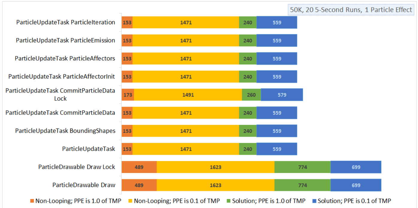
Figure 5.30 A graph showing the number of section calls for various sections of code for a single particle effect. This shows that the Solution data series has fewer section calls than the Non-Looping data series.
