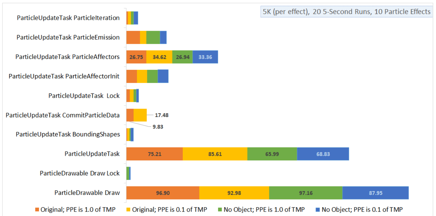
Figure 5.8 A graph showing the time spent in various sections of code for ten particle effects. Like in Figure 5.7, this shows that the Original and No Object data series both have similar run times for the multiple-burst (0.1 TMP) and single-burst (1.0 TMP) games.
