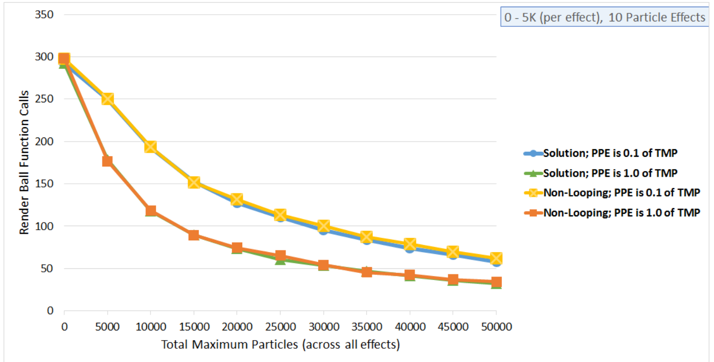
Figure 5.28 A graph showing render ball function calls over total maximum particles for ten particle effects. Since this failure did not occur for many particle effects, we see here that the Solution and Non-Looping data series render the ball about the same number of times.
