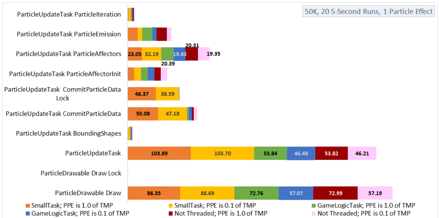
Figure 5.15 A graph showing the time spent in various sections of code for a single particle effect. This shows the Game Logic and Not Threaded data series shared the same run times for the multiple-burst (0.1 TMP) and single-burst (1.0 TMP) games. The Original Data series had longer run times, but this is because it had more opportunities to run (see the section call numbers in Figure 5.14) and not because of poor performance.
