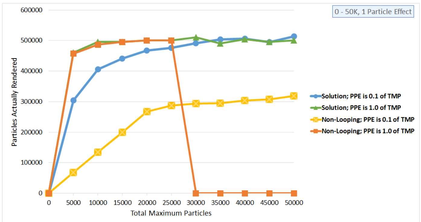
Figure 5.27 A graph showing particles actually rendered over total maximum particles for a single particle effect. This shows that the Solution data series (the one with an increased duration of 120 seconds) does not stop rendering particles to the screen at 30,000 TMP, which is the desired outcome.
