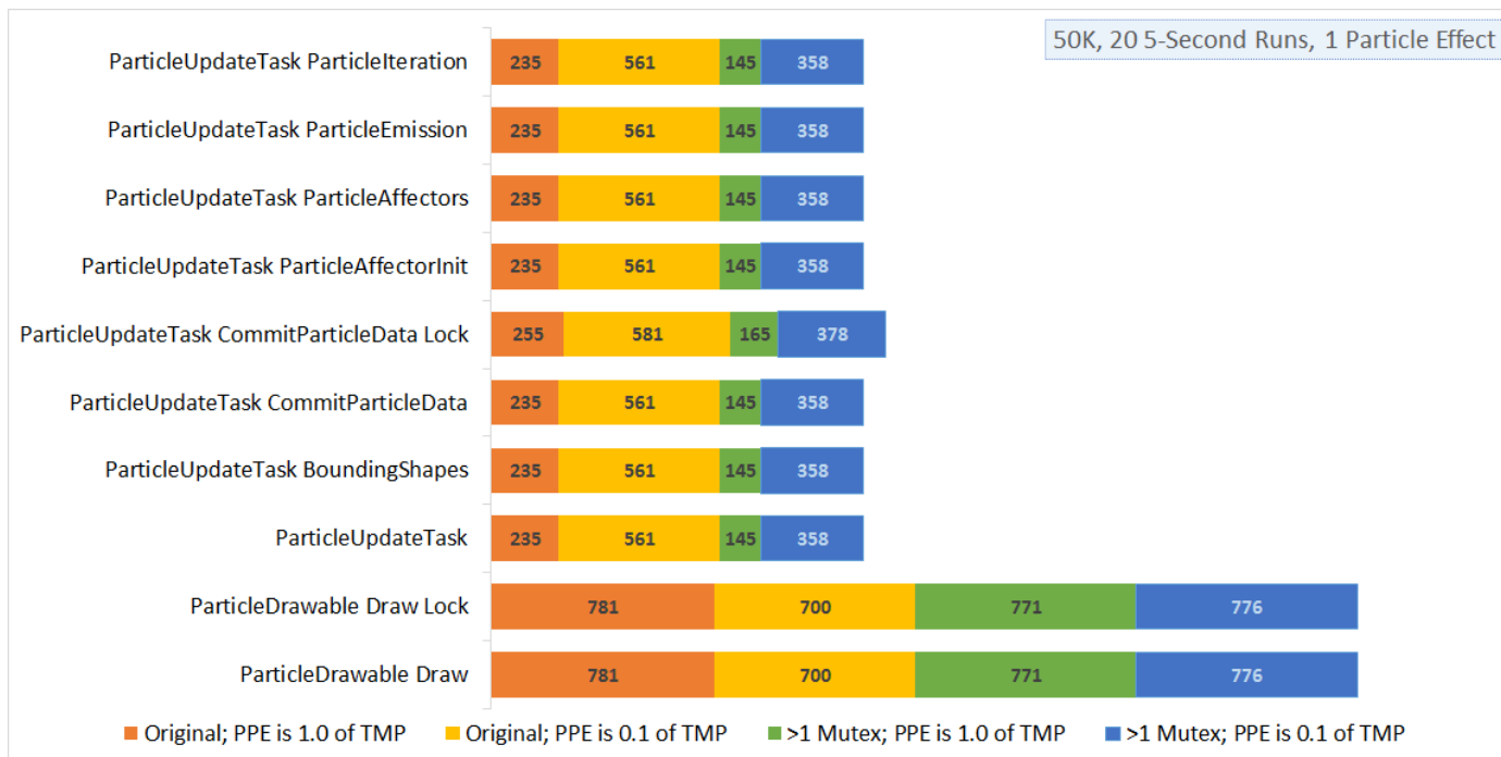
Figure 4.6 A graph showing the number of section calls for various sections of code for a single particle effect. Note that the "ParticleUpdateTask CommitParticleData Lock" section is timing the particle array lock for the > 1 Mutex data series. This shows that, between the > 1 Mutex and Original data series, the drawing functions had approximately the same number of section calls. The Original data series for the particle update functions, however, show more calls.
