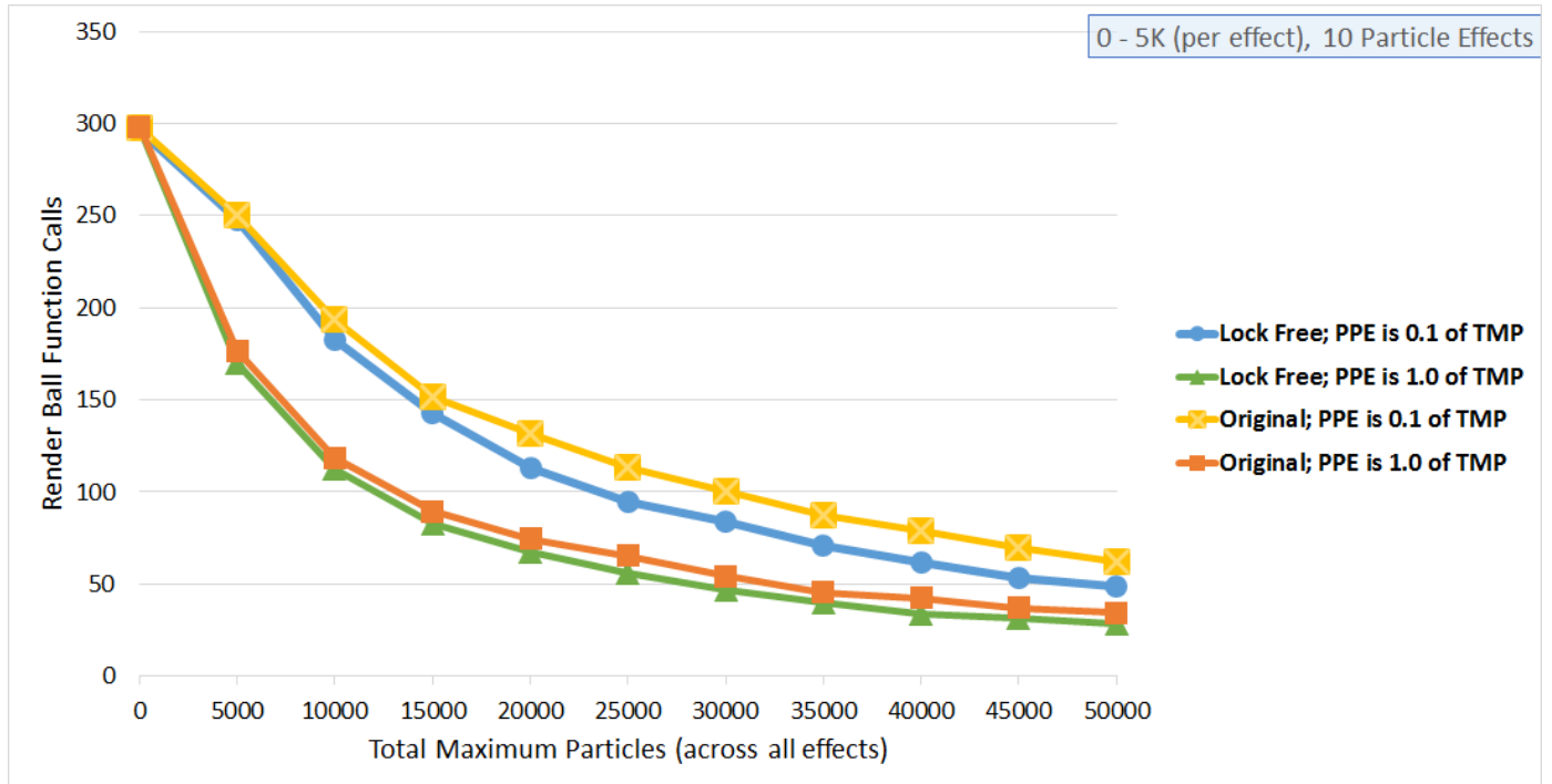
Figure 4.17 A graph showing render ball function calls over total maximum particles for ten particle effects. Although they are very similar, the Lock Free data series exhibits slightly lower render ball function calls values than the Original data series.
