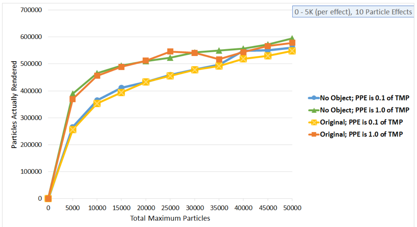
Figure 5.4 A graph showing particles actually rendered over total maximum particles for ten particle effects. Like in Figure 5.3, the particles actually rendered values from the Original and No Object data series are very similar.
