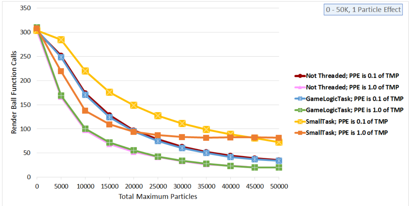
Figure 5.10 A graph showing render ball function calls over total maximum particles for a single particle effect. This shows two things: the Not Threaded and Game Logic Task data series share nearly identical values, and the Small Task data series performs better (i.e. renders the ball more) than the other data series for the multiple-burst (0.1 TMP) and single-burst (1.0 TMP) games.
