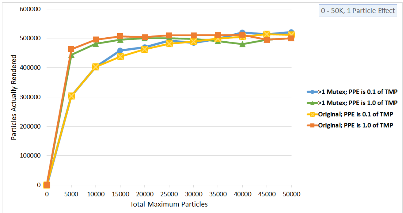
Figure 4.5 A graph showing particles actually rendered over total maximum particles for a single particle effect. This shows that changing Concurrent Particle Data to use multiple mutexes also does not impact the number of times that particles are rendered. As in Figure 4.4, the > 1 Mutex data series is almost the same as the ones for the data series without any changes to the source code (i.e. the Original data series).
