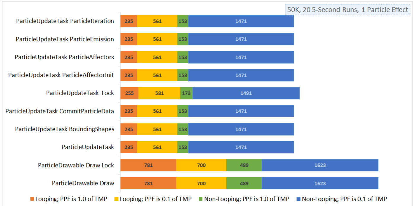
Figure 5.22 A graph showing the number of section calls for various sections of code for a single particle effect. This shows that: (1) The Non-Looping data series in multiple-burst (or 0.1 TMP) games have a significantly higher section call count than the Looping data series, and (2) The Non-Looping data series in single-burst (or 1.0 TMP) games have a lower section call count than the Looping data series.
