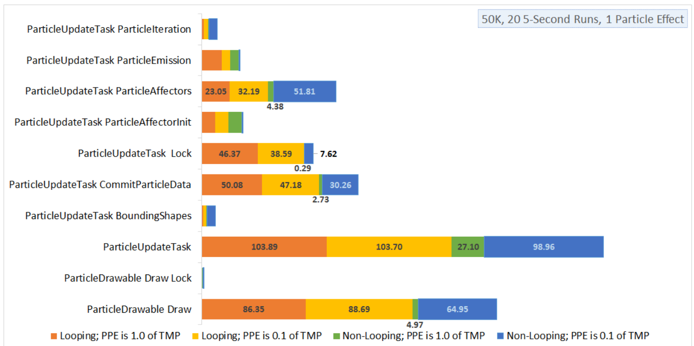
Figure 5.23 A graph showing the time spent in various sections of code for a single particle effect. Similar to Figure 5.22, this shows that: (1) The Non-Looping data series in multiple-burst (or 0.1 TMP) games have a lower run time than the Looping data series, and (2) The Non-Looping data series in single-burst (or 1.0 TMP) games have a significantly lower run time than all of the data series and games.
