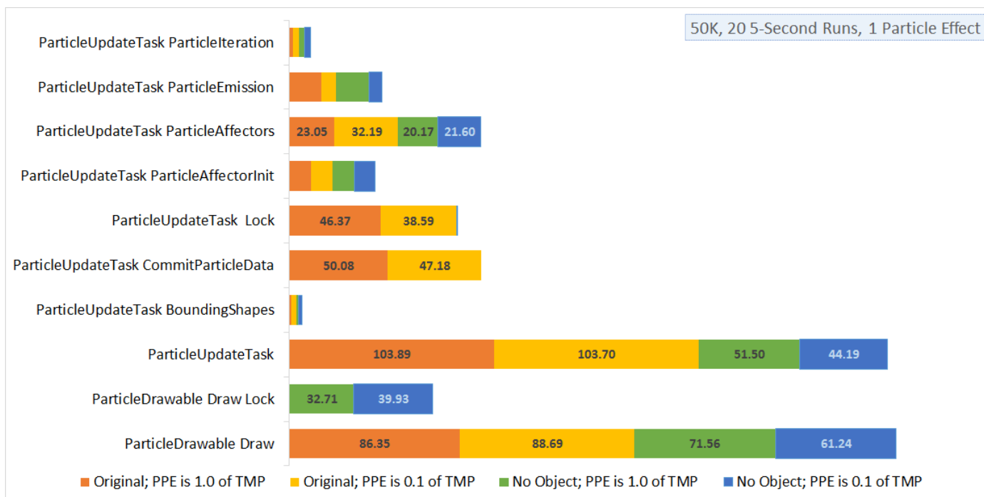
Figure 5.6 A graph showing the time spent in various sections of code for a single particle effect. This illustrates how the contention was moved from CommitParticleData to Draw when the ConcurrentParticleData object was not used (i.e. the No Object data series).
