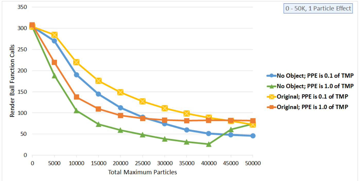
Figure 5.1 A graph showing render ball function calls over total maximum particles for a single particle effect. This shows that the No Object data series exhibits worse performance than the Original data series. The render ball function calls values from the Original data series are consistently higher than the No Object data series for the multiple-burst (0.1 TMP) and single-burst (1.0 TMP) games.
