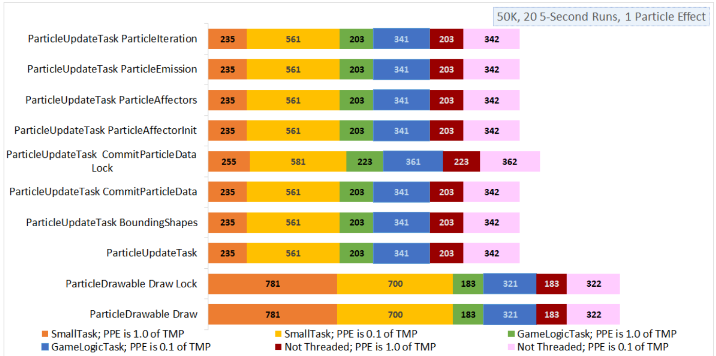
Figure 5.14 A graph showing the number of section calls for various sections of code for a single particle effect. This shows that the Game Logic and Not Threaded data series had about the same number of section calls and that the Original data series had more than both of the other data series for the multiple-burst (0.1 TMP) and single-burst (1.0 TMP) games.
