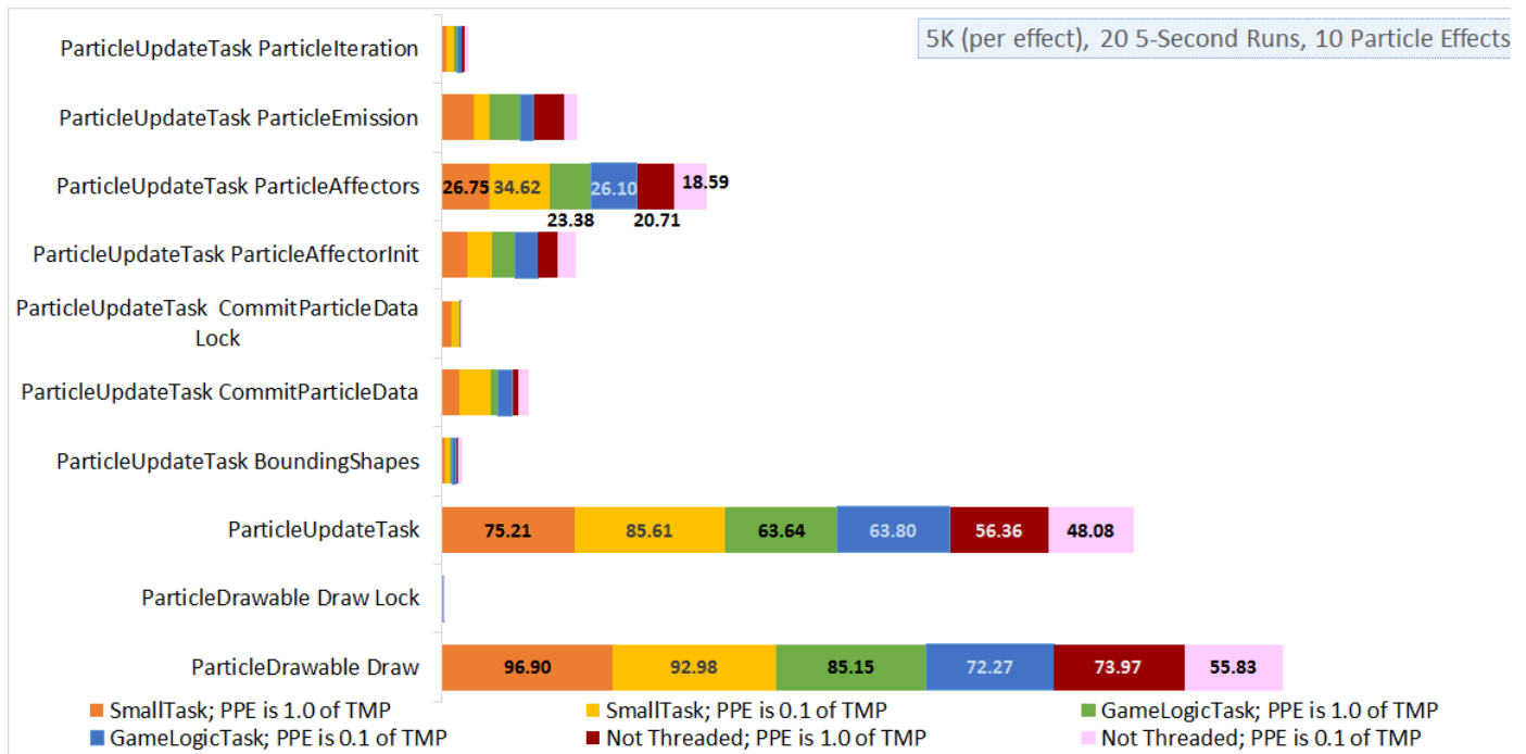
Figure 5.17 A graph showing the time spent in various sections of code for ten particle effects. This shows that the run times between the Game Logic and Not Threaded data series are not terribly different, but Not Threaded does have slightly lower run times than the Game Logic Task. Although a lower run time usually indicates better performance, in this case this is not true when we weigh this fact against Figures 5.12 and 5.13. This is because lower render ball function calls value results in choppy visuals, and that is not at all desirable to the end-user.
