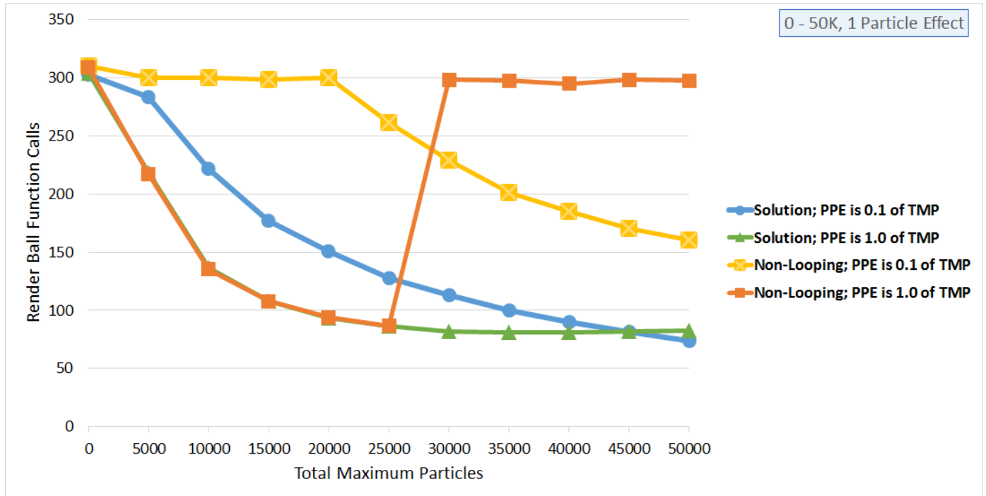
Figure 5.26 A graph showing render ball function calls over total maximum particles for a single particle effect. This shows that the Solution data series (the one with an increased duration of 120 seconds) does not spike in performance at 30,000 TMP. This is a good thing because it means that the renderer was spending some of its time rendering particles (see Figure 5.29).
