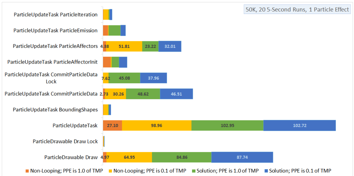
Figure 5.31 A graph showing the time spent in various sections of code for a single particle effect. This shows that the Solution data series has overall longer run times than the Non-Looping data series; this is because the Particle Effect Component is actually being rendered and processed instead of being stopped early on in the game.
