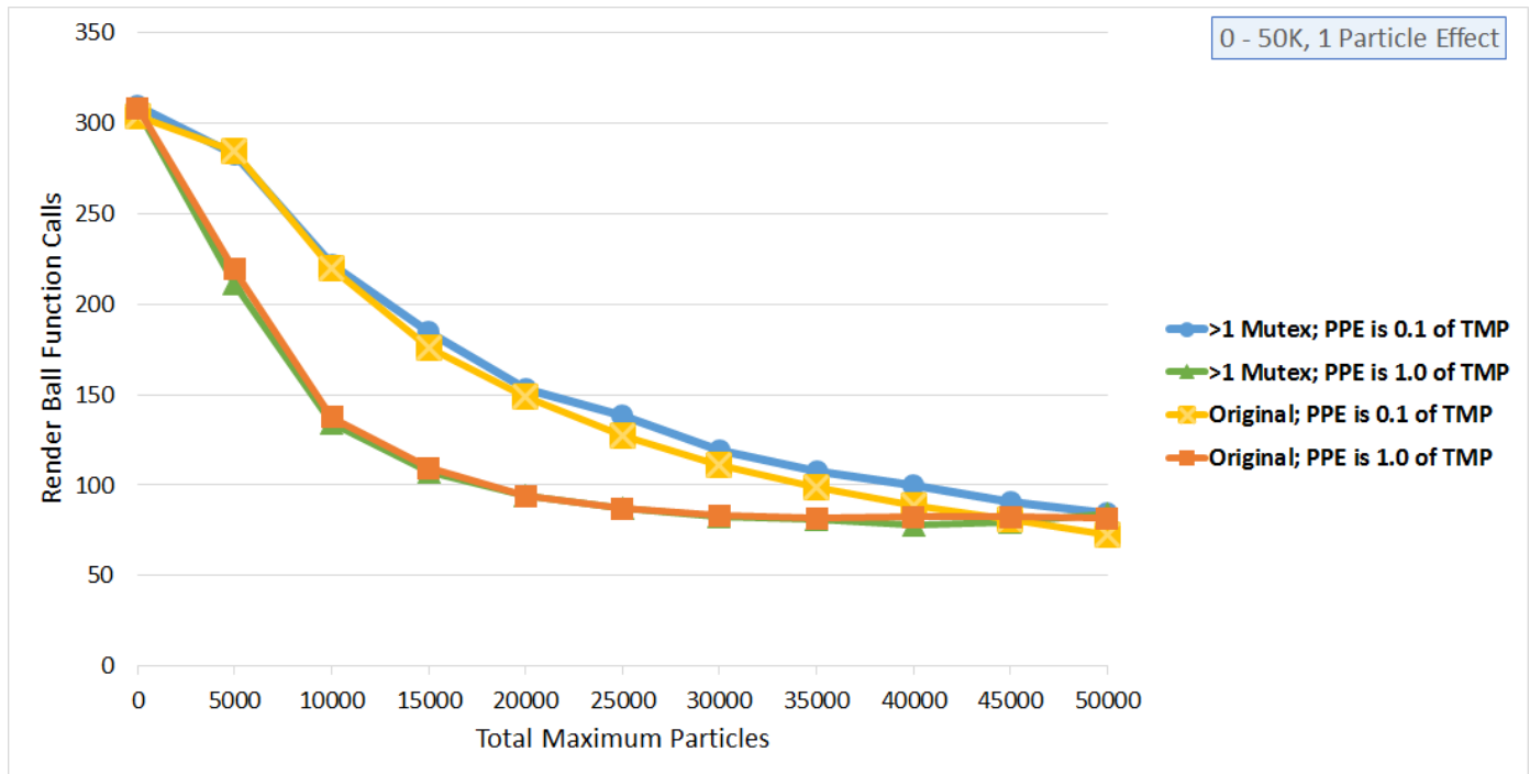
Figure 4.4 A graph showing render ball function calls over total maximum particles for a single particle effect. This shows that changing Concurrent Particle Data to use multiple mutexes does not impact the number of times that the ball is rendered. The multiple-burst and single-burst (0.1 and 1.0 TMP, respectively) scenarios for the > 1 Mutex data series are almost the same as the ones for the data series without any changes to the source code (i.e. the Original data series).
