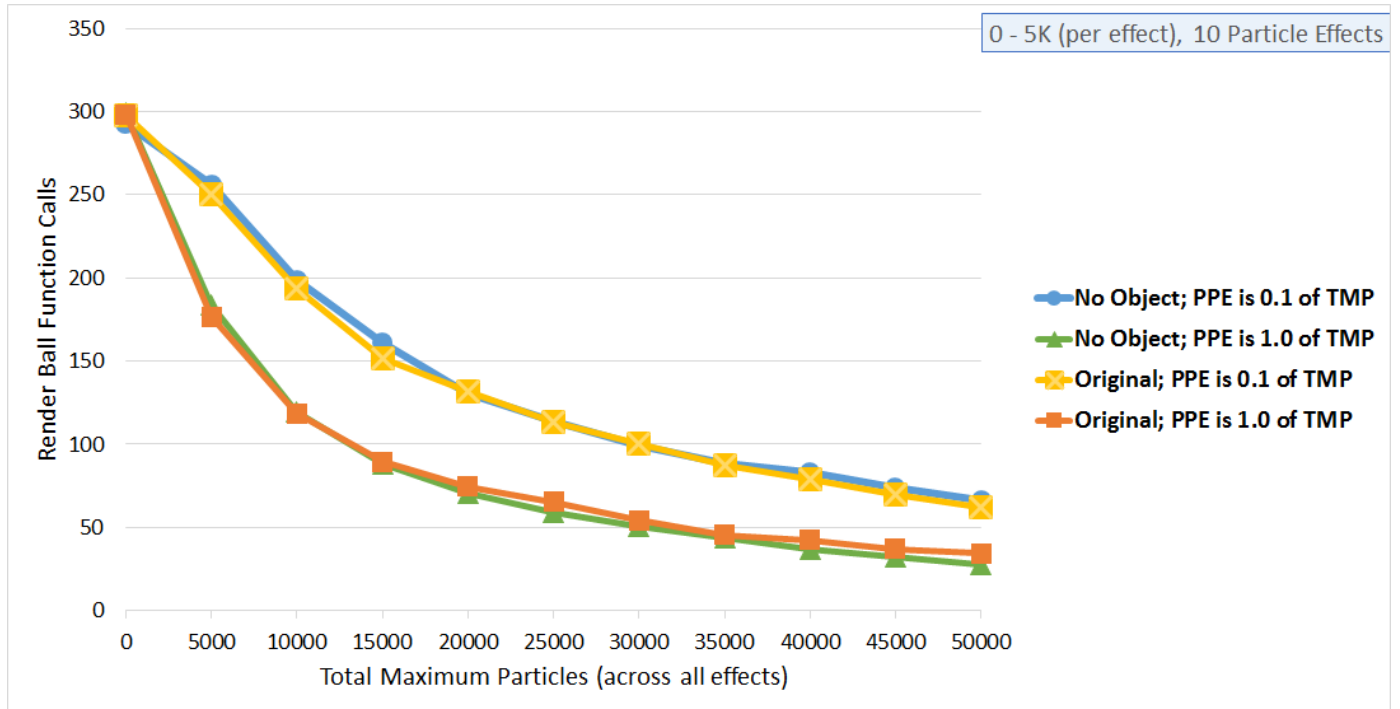
Figure 5.3 A graph showing render ball function calls over total maximum particles for ten particle effects. This shows little to no difference between the render ball function calls values from the Original and No Object data series for the multiple-burst (0.1 TMP) and single-burst (1.0 TMP) games.
