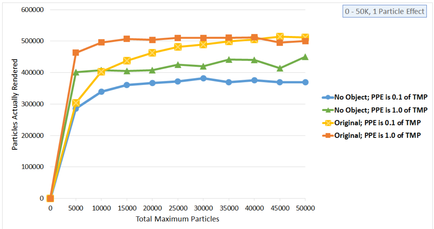
Figure 5.2 A graph showing particles actually rendered over total maximum particles for a single particle effect. Similarly to Figure 5.1, this shows that the Original data series performs better (i.e. renders more particles) than the No Object data series for the multiple-burst (0.1 TMP) and single-burst (1.0 TMP) games.
