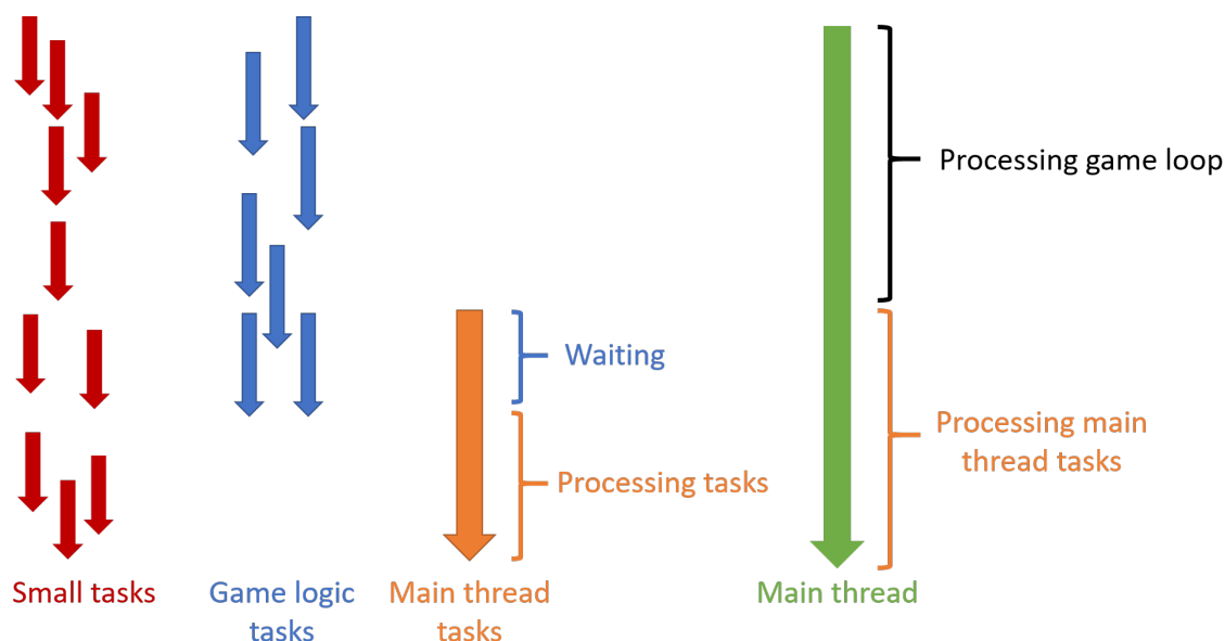
Figure 5.9: Illustrates the lifetime of small tasks , game logic tasks , and main thread tasks in relation to the main thread. The important concept to understand from this figure is how small tasks are ran whenever regardless of what the main thread is doing and the main thread tasks are bound by the main thread. The game logic tasks can also be technically ran as the main thread is processing the game loop, but it is special in that it is guaranteed to be done by the end of the current frame.
