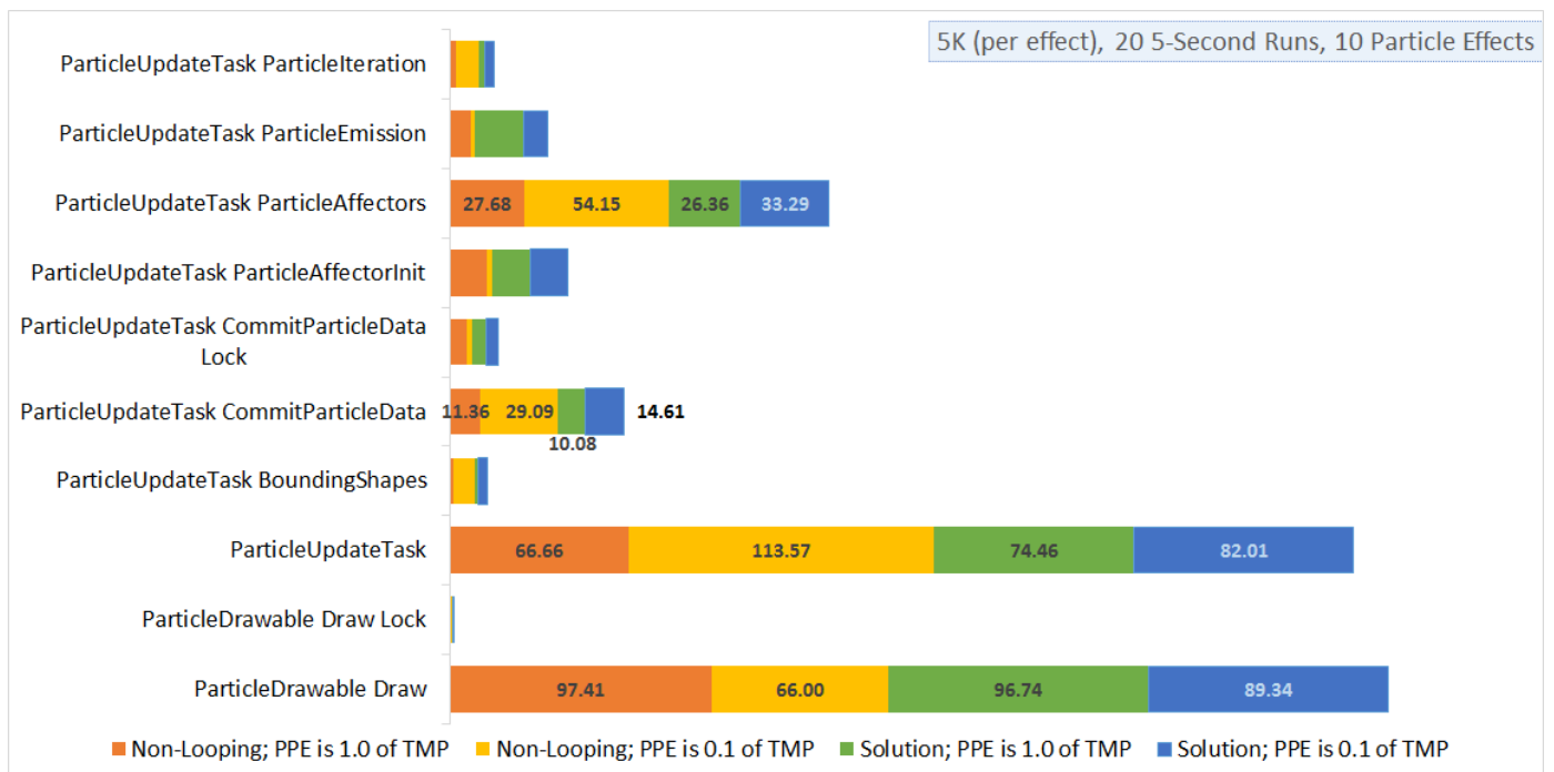
Figure 5.33 A graph showing the time spent in various sections of code for ten particle effects. This shows: (1) The multiple-burst (or 0.1 TMP) games for the Non-Looping data series has a higher run time for particle update functions and a lower run time for particle draw functions than the Solution data series, and (2) The single-burst (or 1.0 TMP) games for the Non-Looping and Solution data series both have approximately the same run time.
