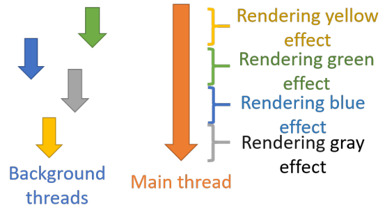
Figure 4.24 The lifetime of a many particle effects in relation to their scheduled background threads and the main thread.
