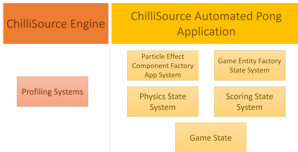
Figure 3.2: The basic architecture of the automated pong game.
