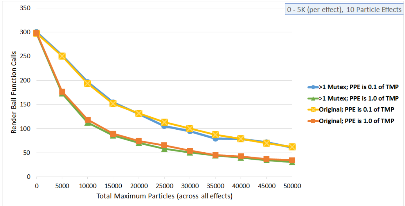
Figure 4.13 A graph showing render ball function calls over total maximum particles for ten particle effects. The two data series, > 1 Mutex and Original, show no stark differences; their render ball function calls values are nearly the same for the multiple-burst (0.1 TMP) and single-burst (1.0 TMP) games.
