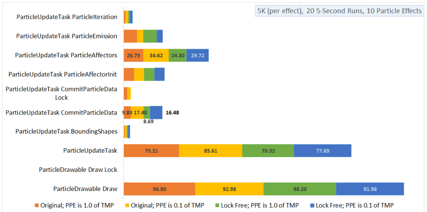
Figure 4.20 A graph showing the time spent in various sections of code for ten particle effects. Unlike in the single particle effect results, this shows not only no significant improvement to the CommitParticleData function, but it also shows that there was little contention to begin with in the Original data series.
