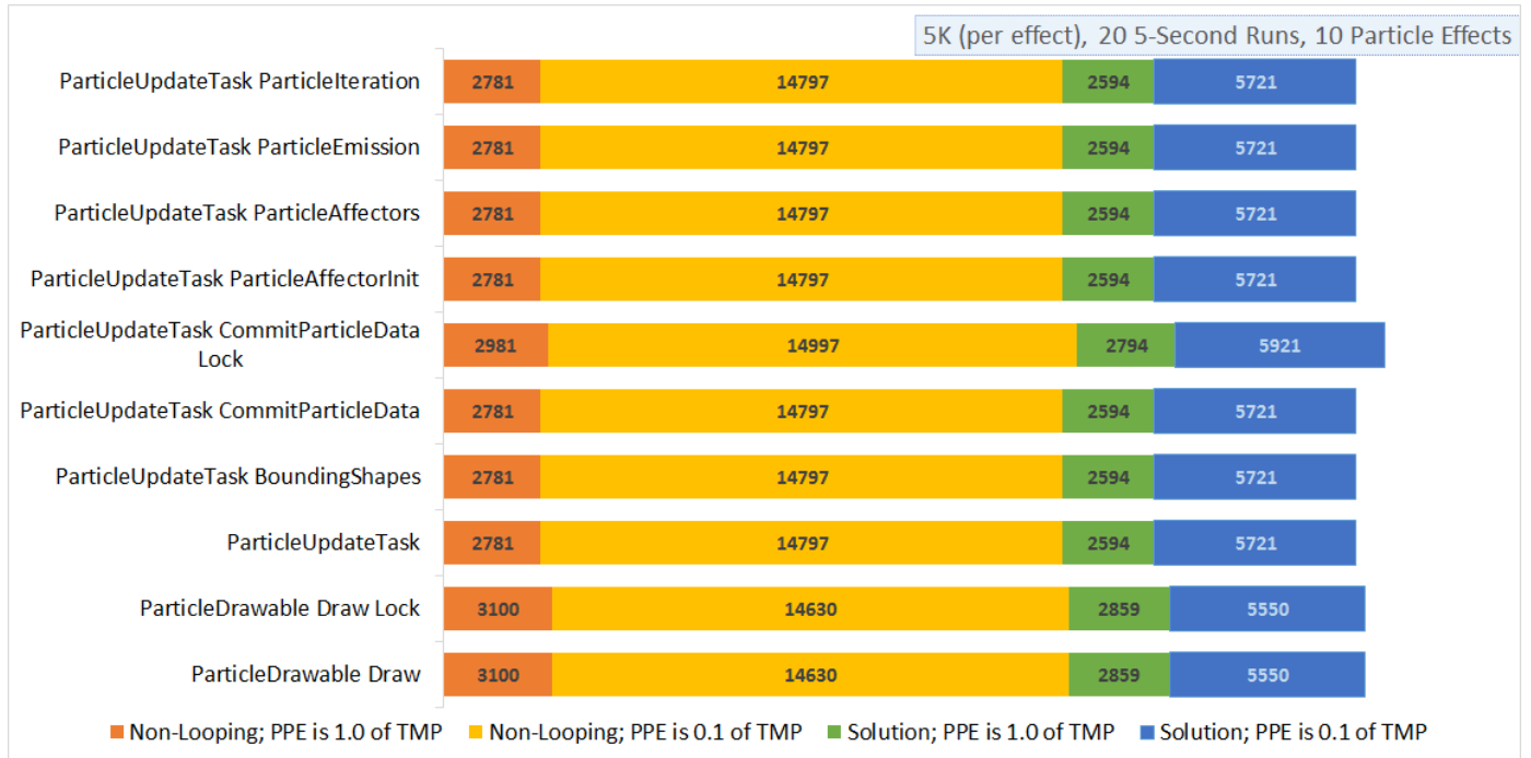
Figure 5.32 A graph showing the number of section calls for various sections of code for ten particle effects. This shows: (1) The multiple-burst (or 0.1 TMP) games for the Non-Looping data series has significantly more section calls than the Solution data series, and (2) The single-burst (or 1.0 TMP) games for the Non-Looping data series has a little more section calls than the Solution data series, but their values are fairly similar.
