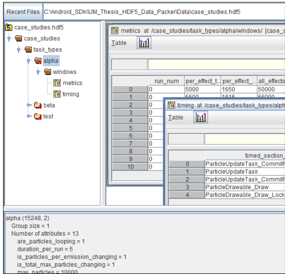
Figure 4.13: An example of an HDF5 file containing sample metrics, timing, and metadata information.
