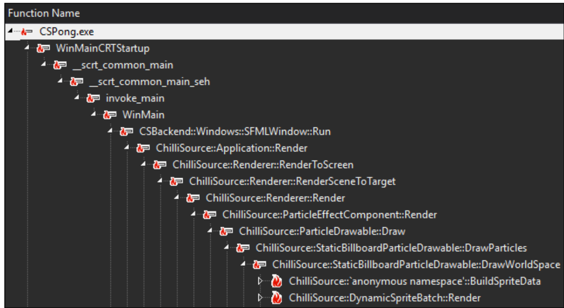
Figure 4.8 Shows an example of Visual Studio's generated call tree for CPU instrumentation when ran using the metadata from Figure 4.2.
