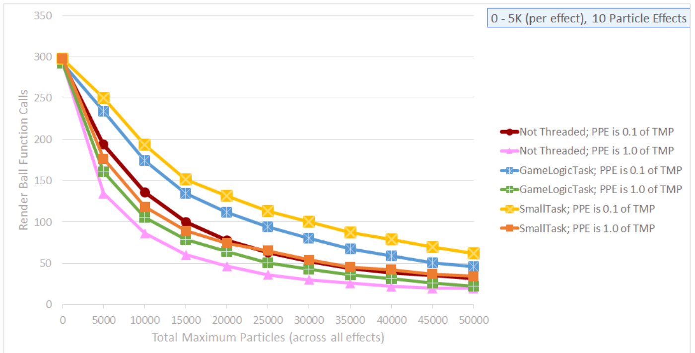
Figure 6.11 A graph showing render ball function calls over total maximum particles for ten particle effects.
