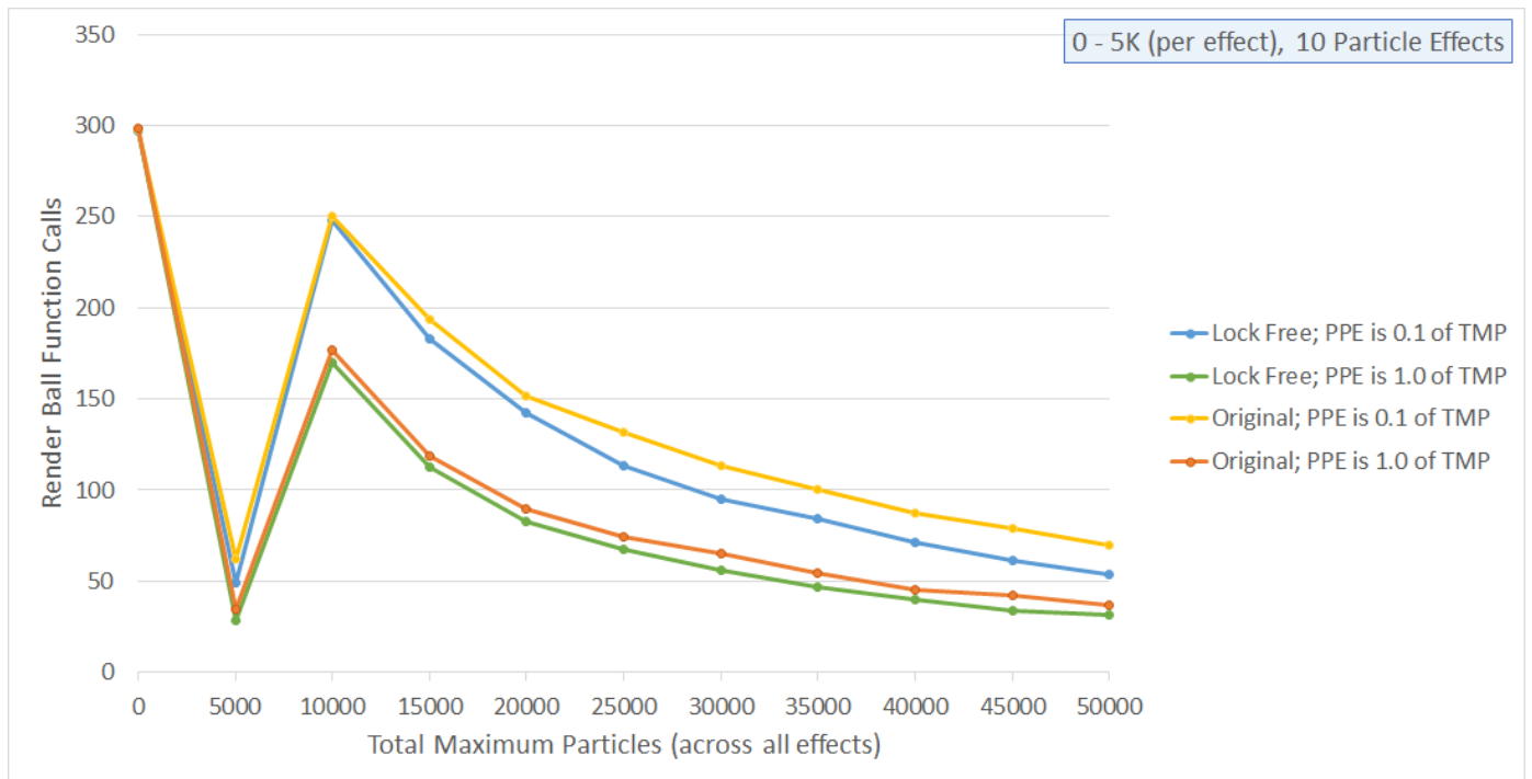
Figure 5.14 A graph showing render ball function calls over total maximum particles for a ten particle effects.
