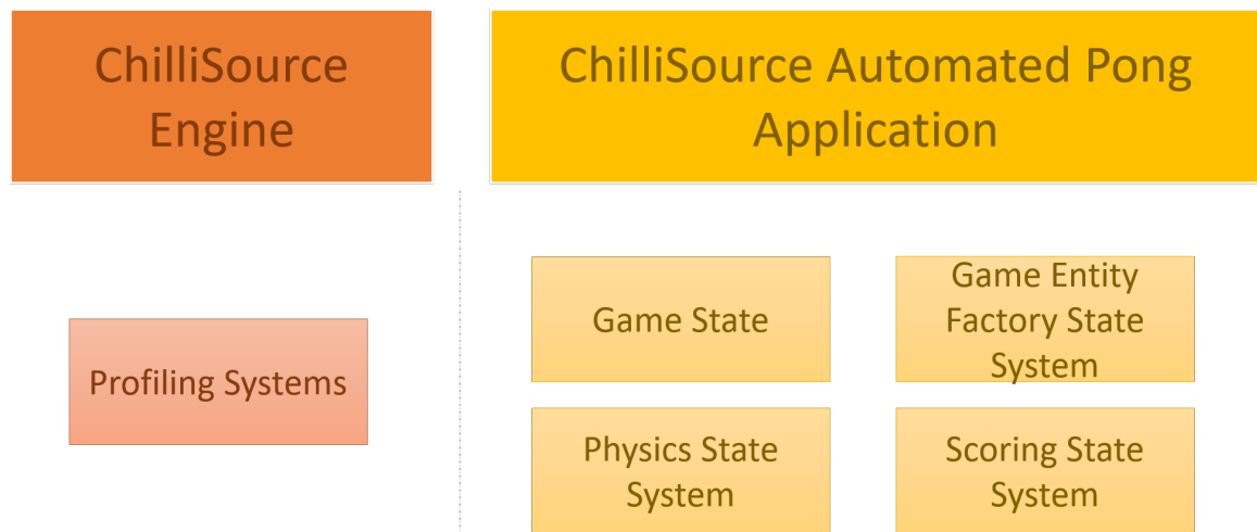
Figure 3.1: The basic architecture of the automated pong game.
