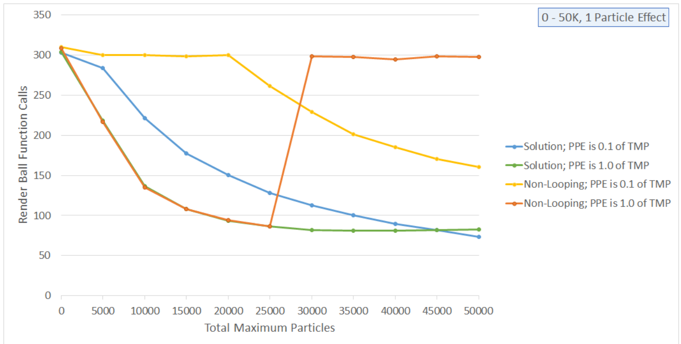
Figure 6.21 A graph showing render ball function calls over total maximum particles for a single particle effect.
