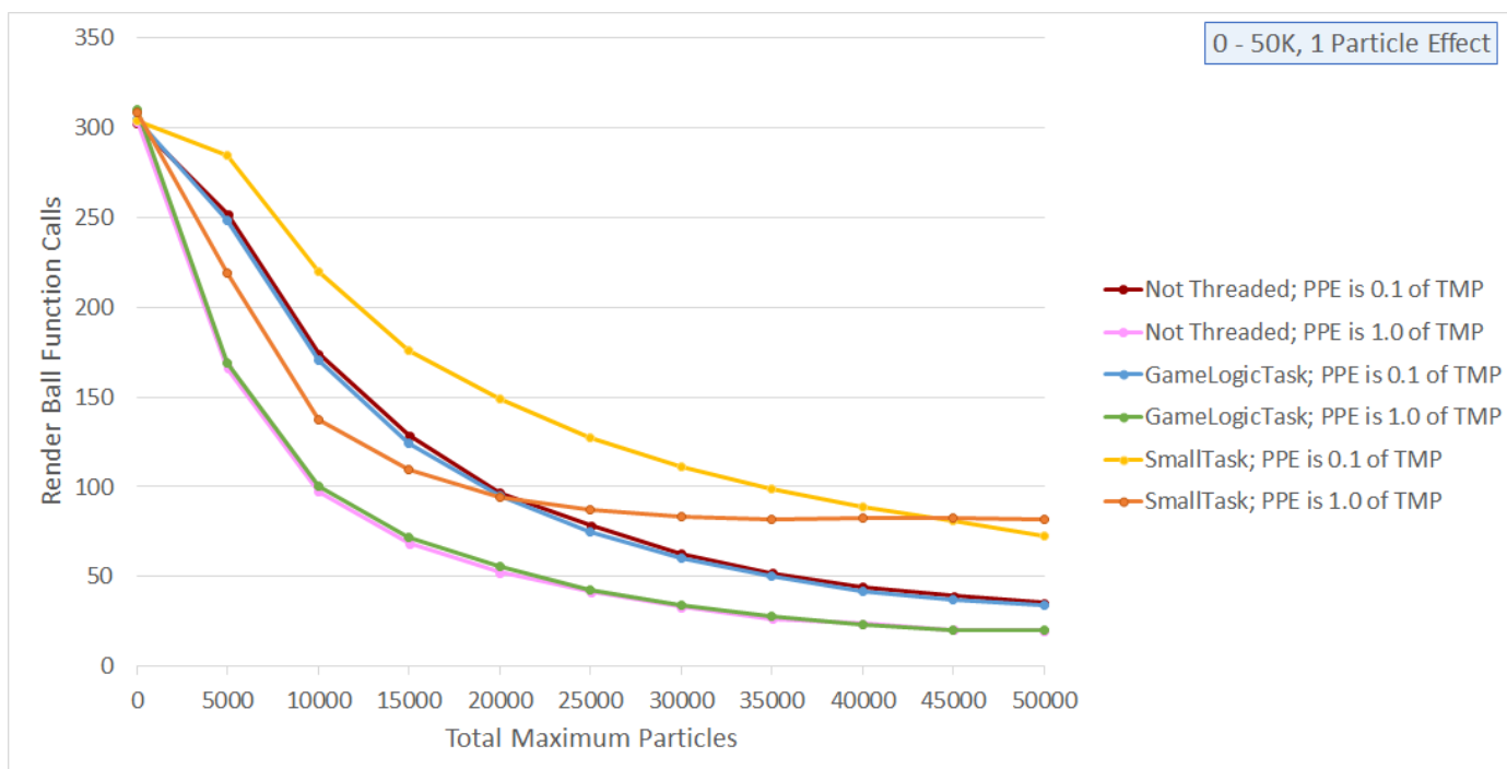
Figure 6.9 A graph showing render ball function calls over total maximum particles for a single particle effect.
