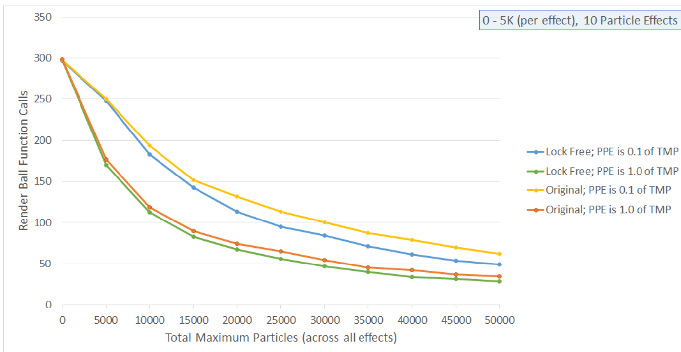
Figure 5.16 A graph showing render ball function calls over total maximum particles for a ten particle effects.
