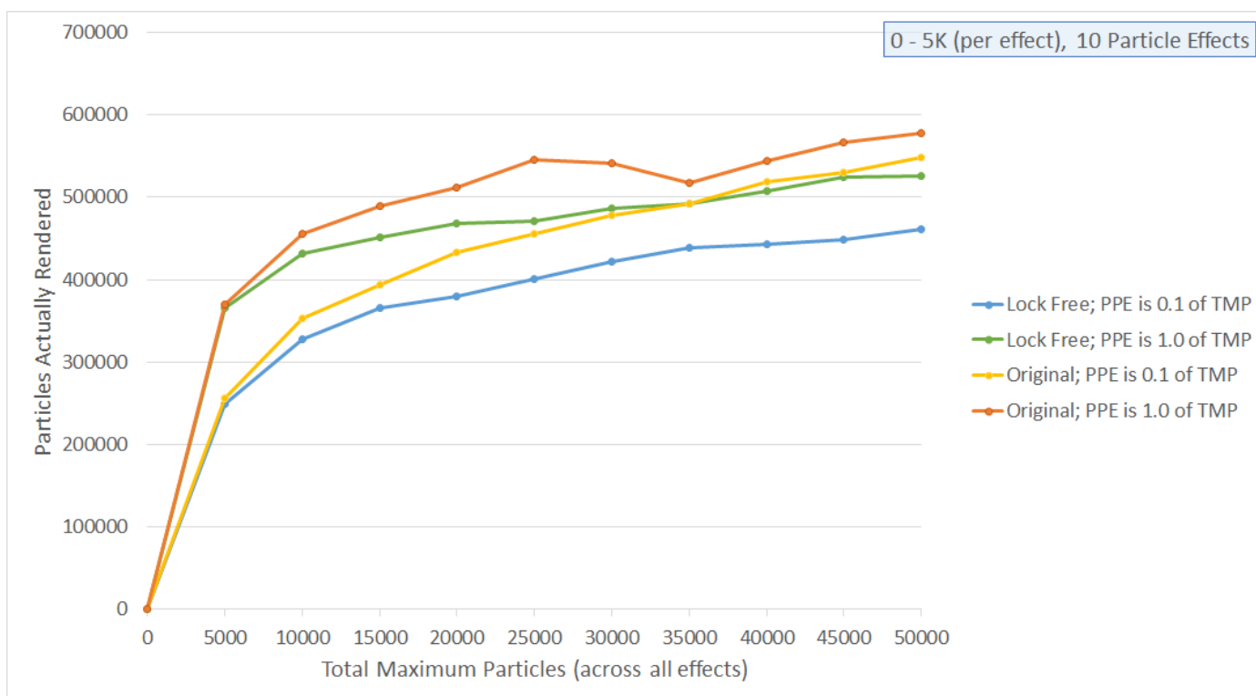
Figure 5.17 A graph showing particles actually rendered over total maximum particles for a ten particle effects.
