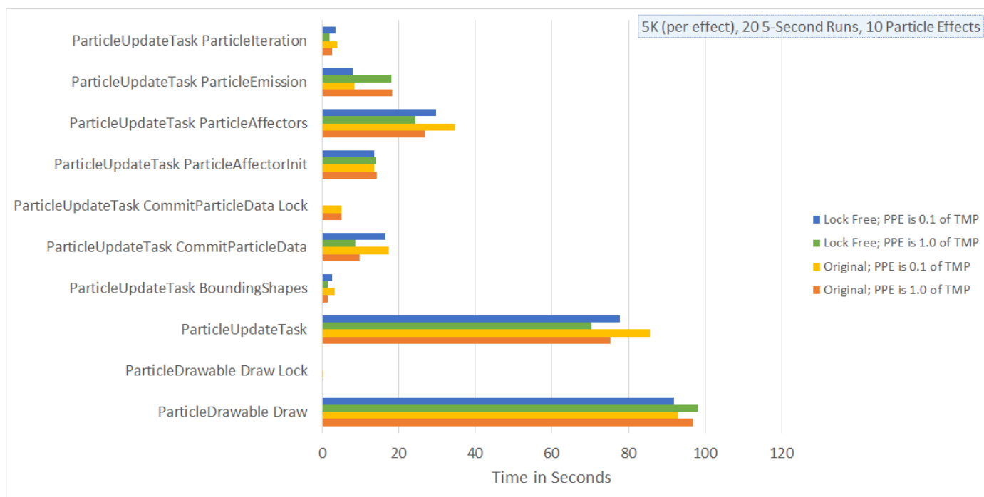
Figure 5.19 A graph showing the time spent in various sections of code for a ten particle effects.
