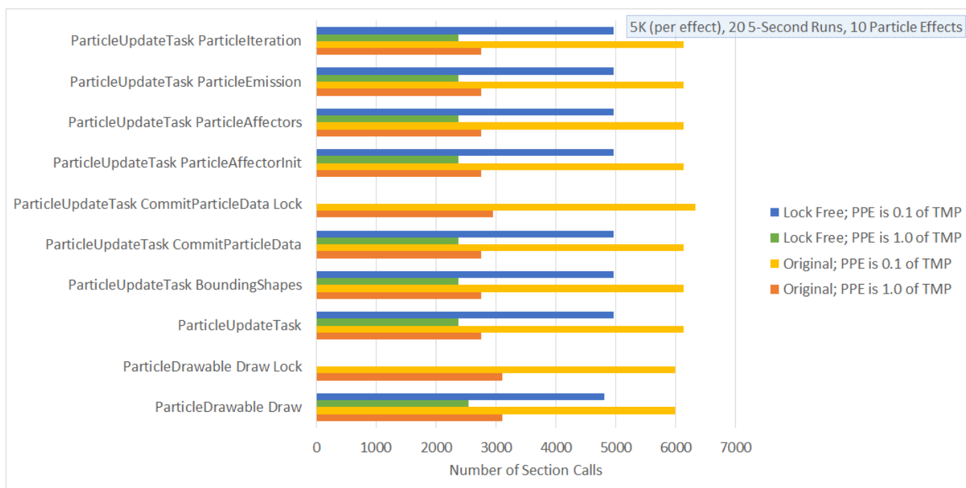
Figure 5.18 A graph showing the number of section calls for various sections of code for a ten particle effects.
