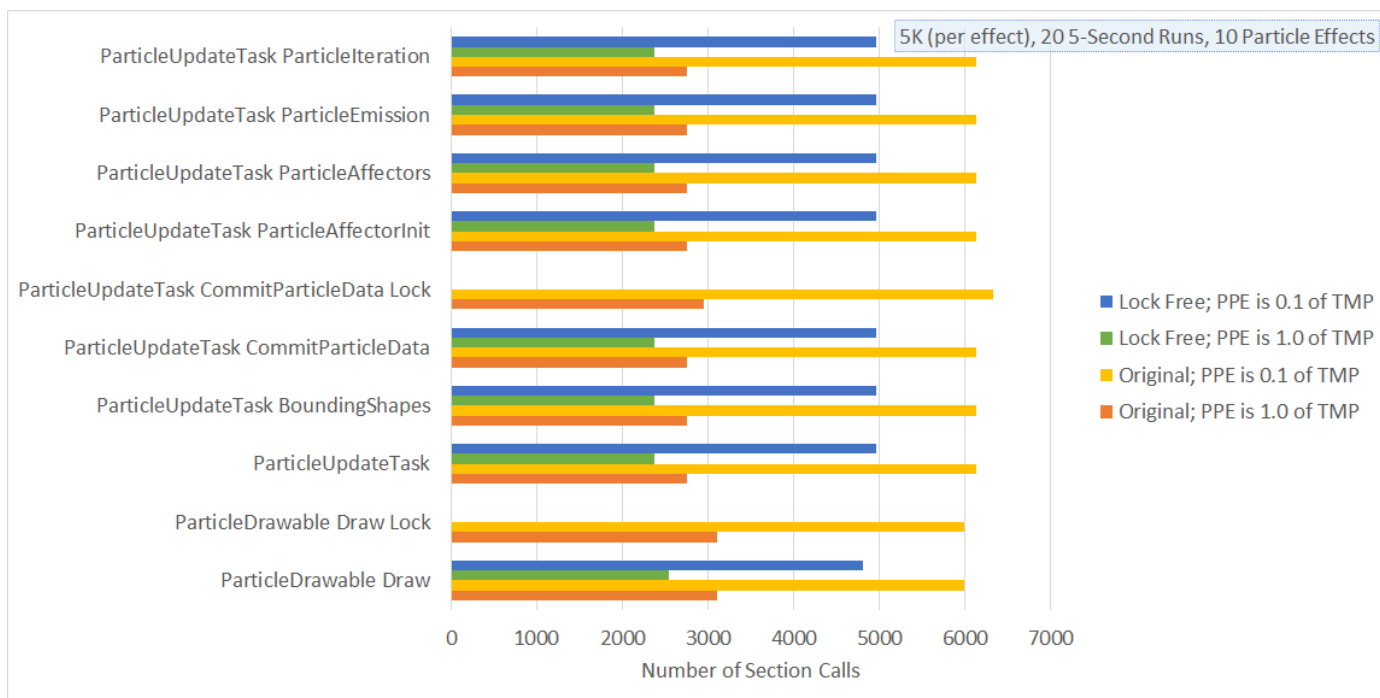
Figure 5.15 A graph showing the number of section calls for various sections of code for a ten particle effects.
