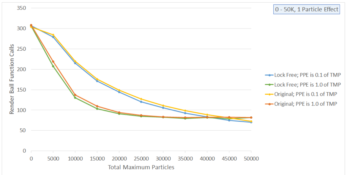
Figure 5.5 A graph showing render ball function calls over total maximum particles for a single particle effect.
