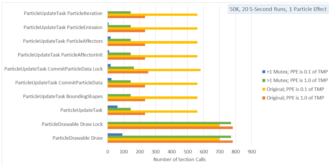
Figure 5.3 A graph showing the number of section calls for various sections of code for a single particle effect.
