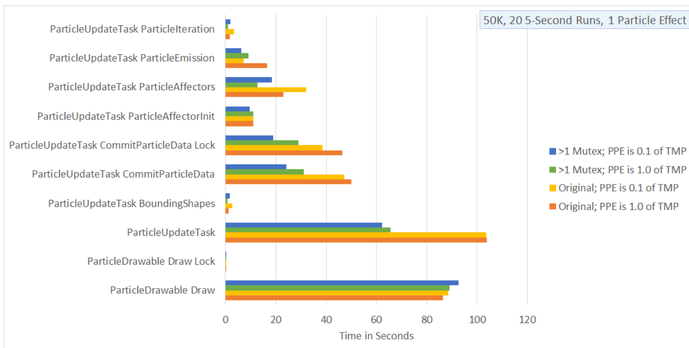
Figure 5.4 A graph showing the time spent in various sections of code for a single particle effect.
