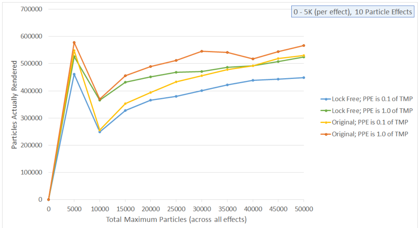
Figure 5.14 A graph showing particles actually rendered over total maximum particles for a ten particle effects.
