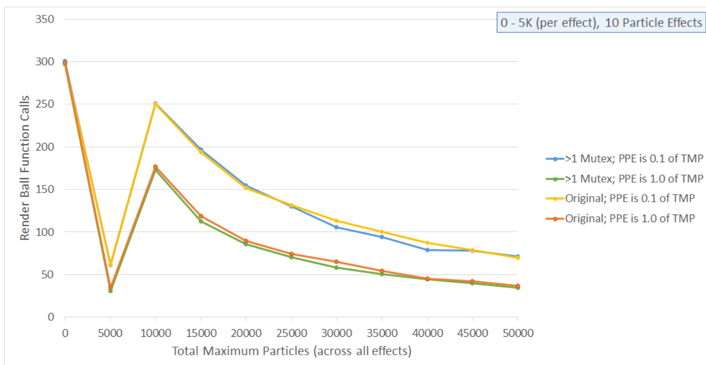
Figure 5.9 A graph showing render ball function calls over total maximum particles for ten particle effects.
