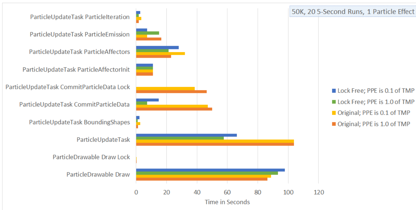
Figure 5.8 A graph showing the time spent in various sections of code for a single particle effect.
