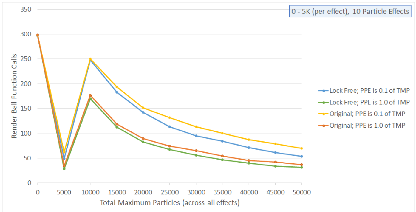
Figure 5.13 A graph showing render ball function calls over total maximum particles for a ten particle effects.
