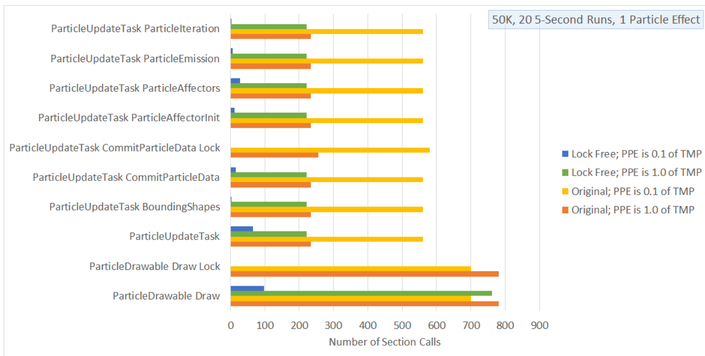
Figure 5.7 A graph showing the number of section calls for various sections of code for a single particle effect.
