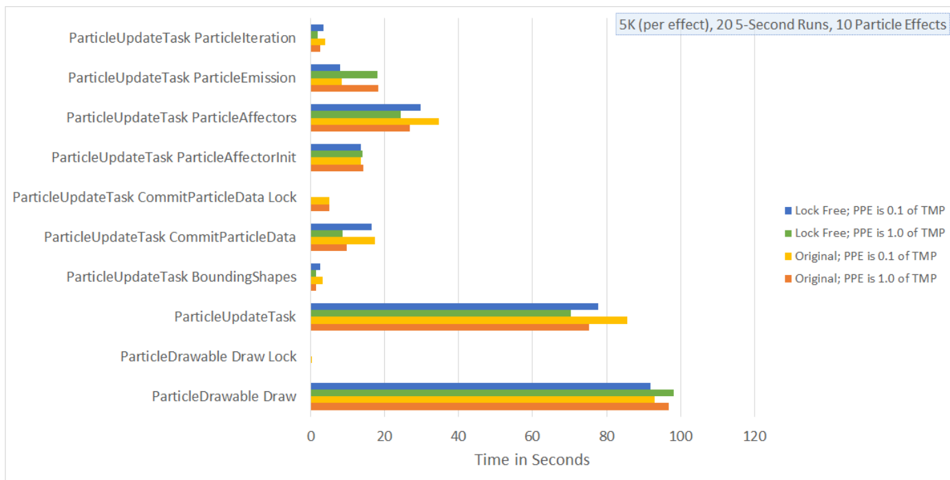
Figure 5.16 A graph showing the time spent in various sections of code for a ten particle effects.
