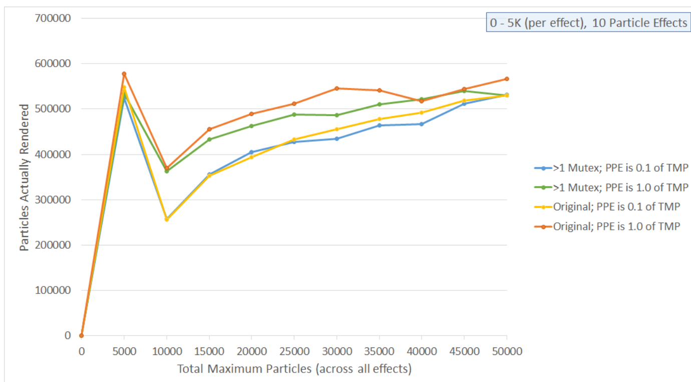
Figure 5.10 A graph showing particles actually rendered over total maximum particles for ten particle effects.
