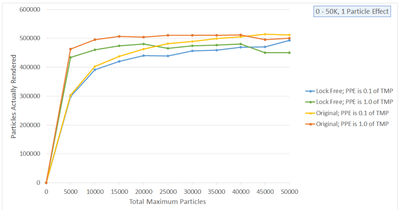
Figure 5.6 A graph showing particles actually rendered over total maximum particles for a single particle effect.
