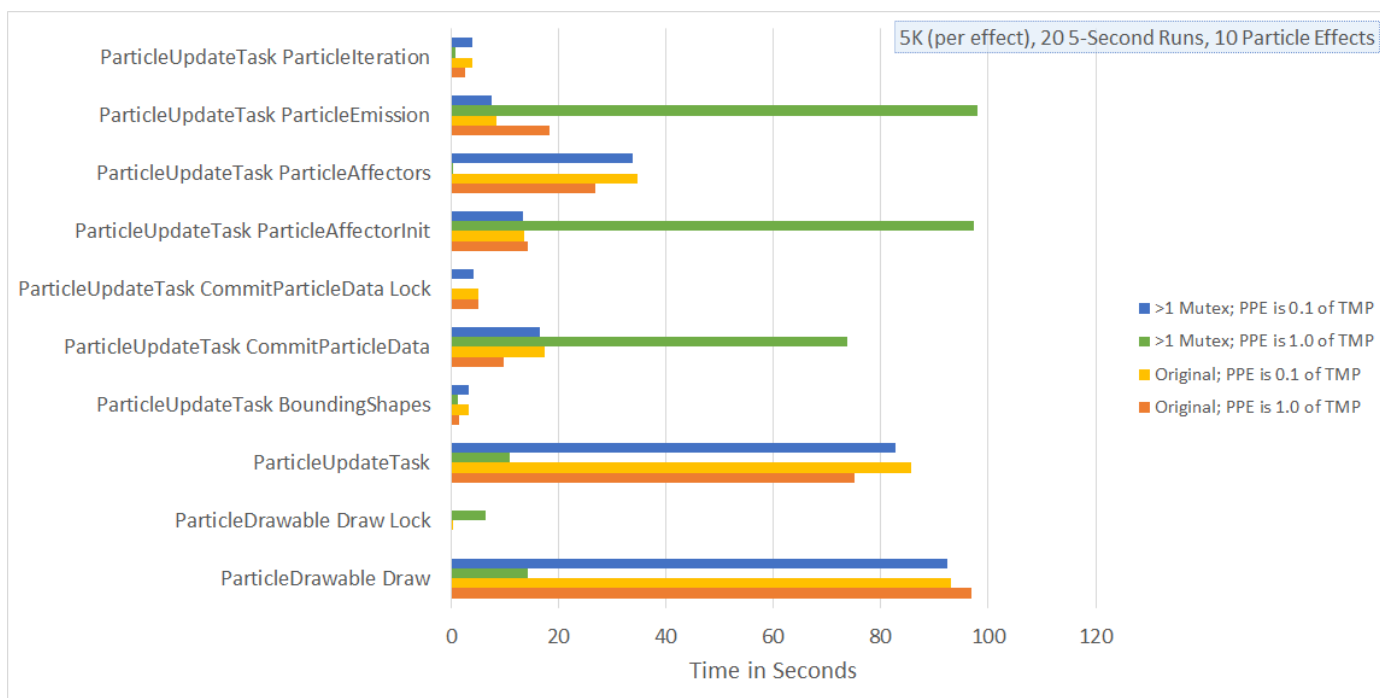
Figure 5.13 A graph showing the time spent in various sections of code for ten particle effects.
