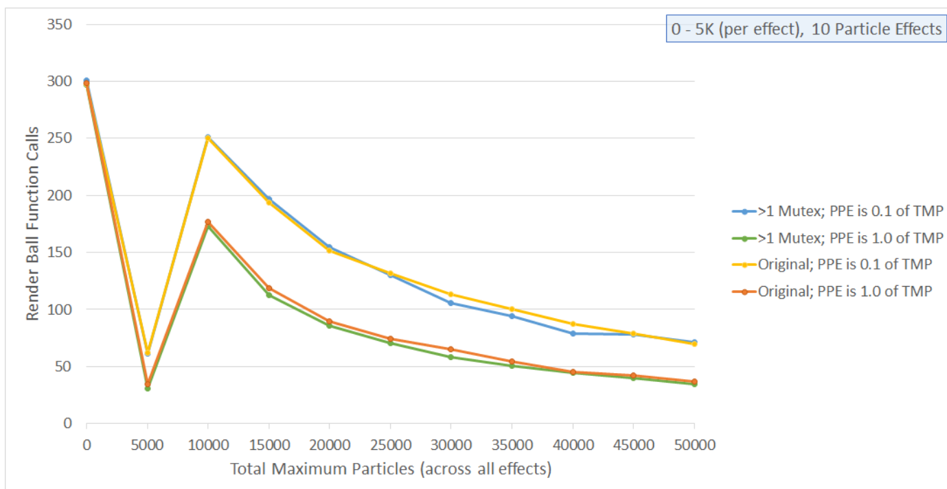
Figure 5.10 A graph showing render ball function calls over total maximum particles for ten particle effects.
