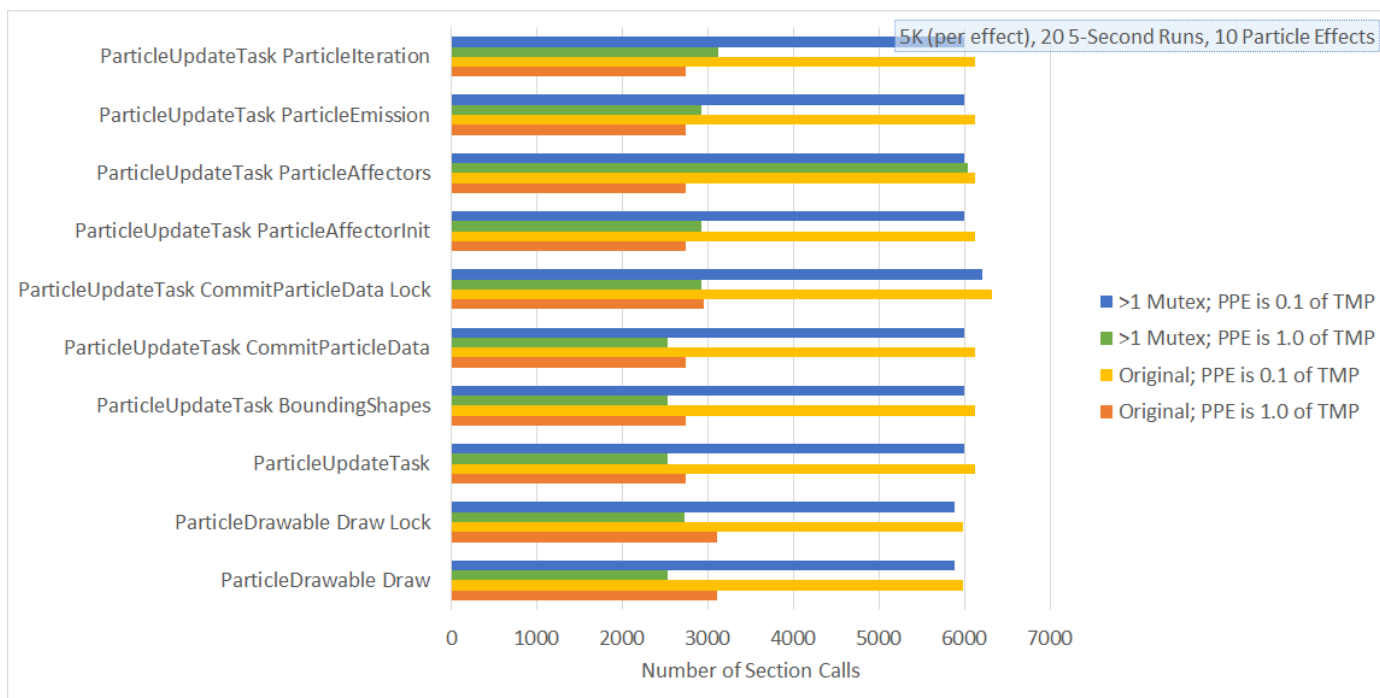
Figure 5.12 A graph showing the number of section calls for various sections of code for ten particle effects.
