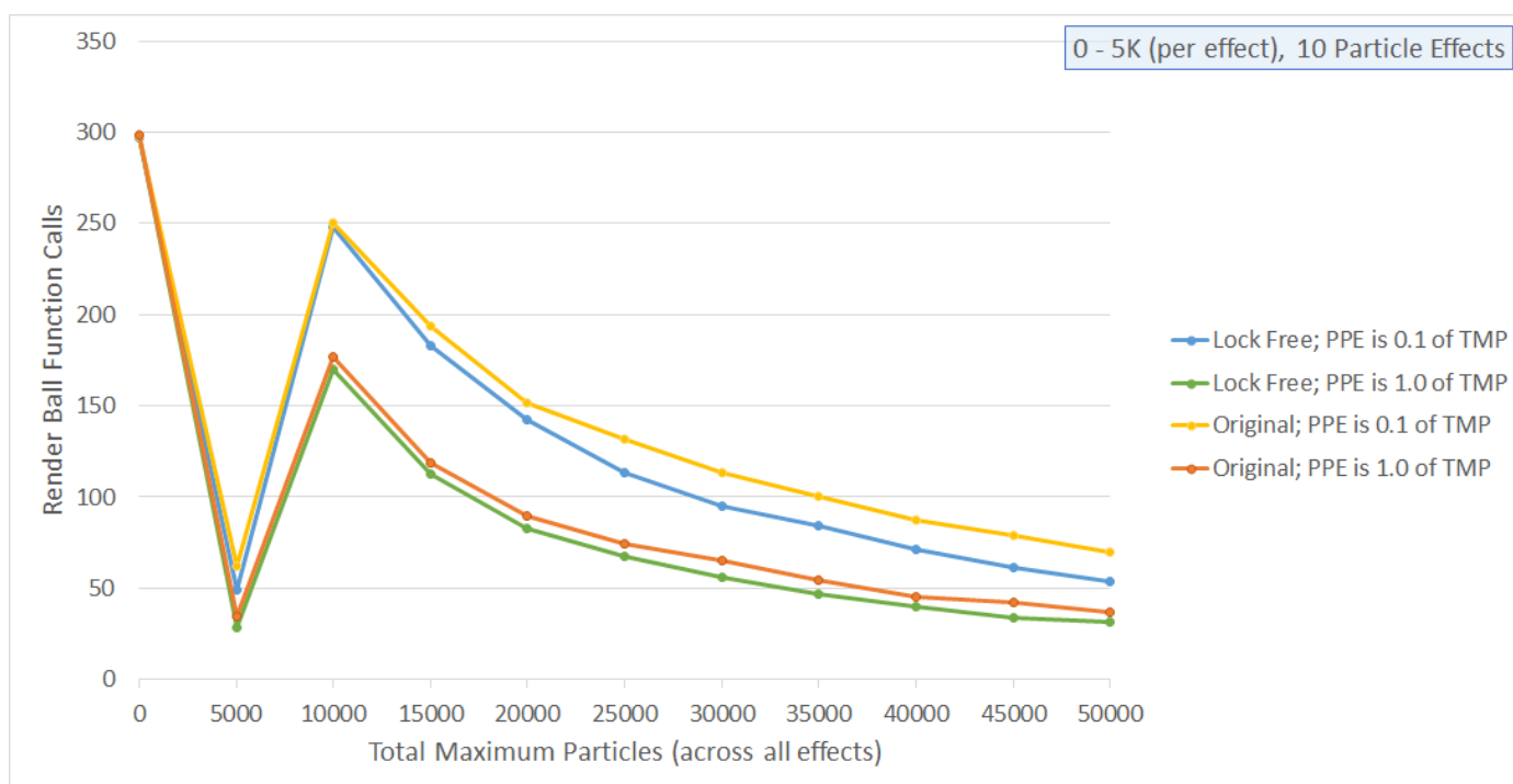
Figure 5.14 A graph showing render ball function calls over total maximum particles for a ten particle effects.
