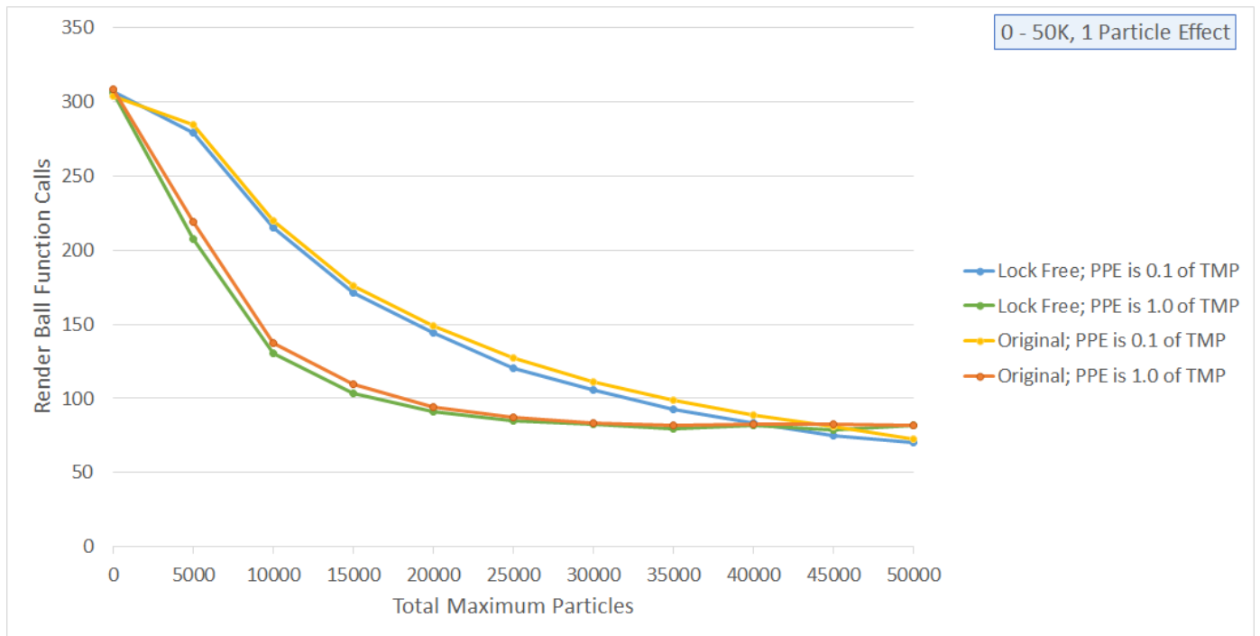
Figure 5.6 A graph showing render ball function calls over total maximum particles for a single particle effect.
