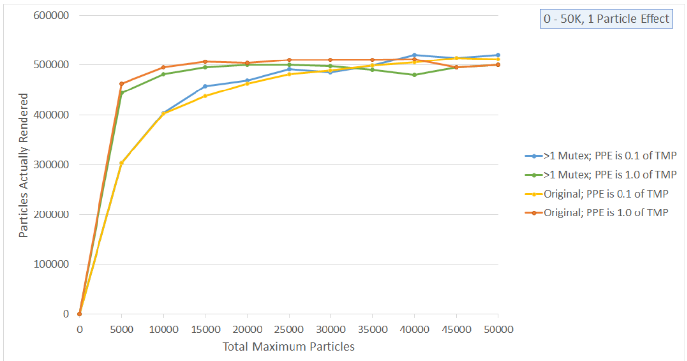
Figure 5.3 A graph showing particles actually rendered over total maximum particles for a single particle effect.
