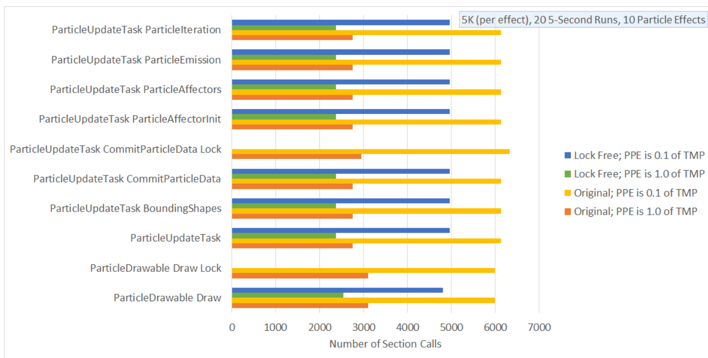
Figure 5.16 A graph showing the number of section calls for various sections of code for a ten particle effects.
