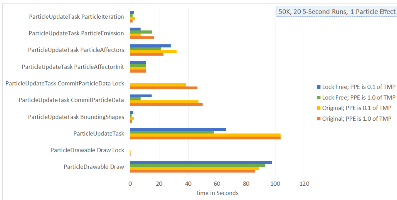
Figure 5.9 A graph showing the time spent in various sections of code for a single particle effect.
