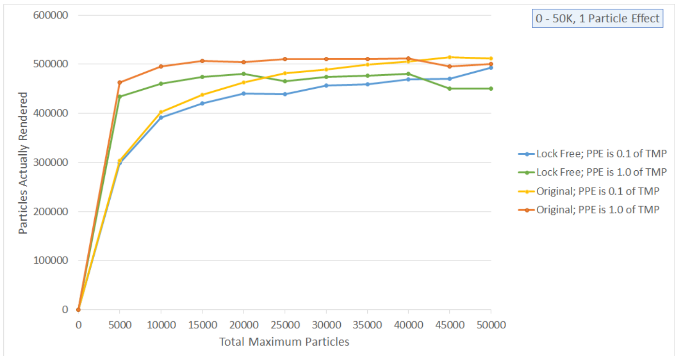
Figure 5.7 A graph showing particles actually rendered over total maximum particles for a single particle effect.
