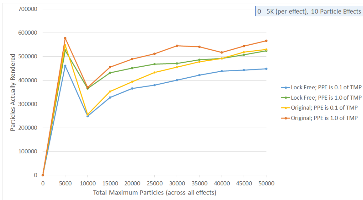
Figure 5.15 A graph showing particles actually rendered over total maximum particles for a ten particle effects.
