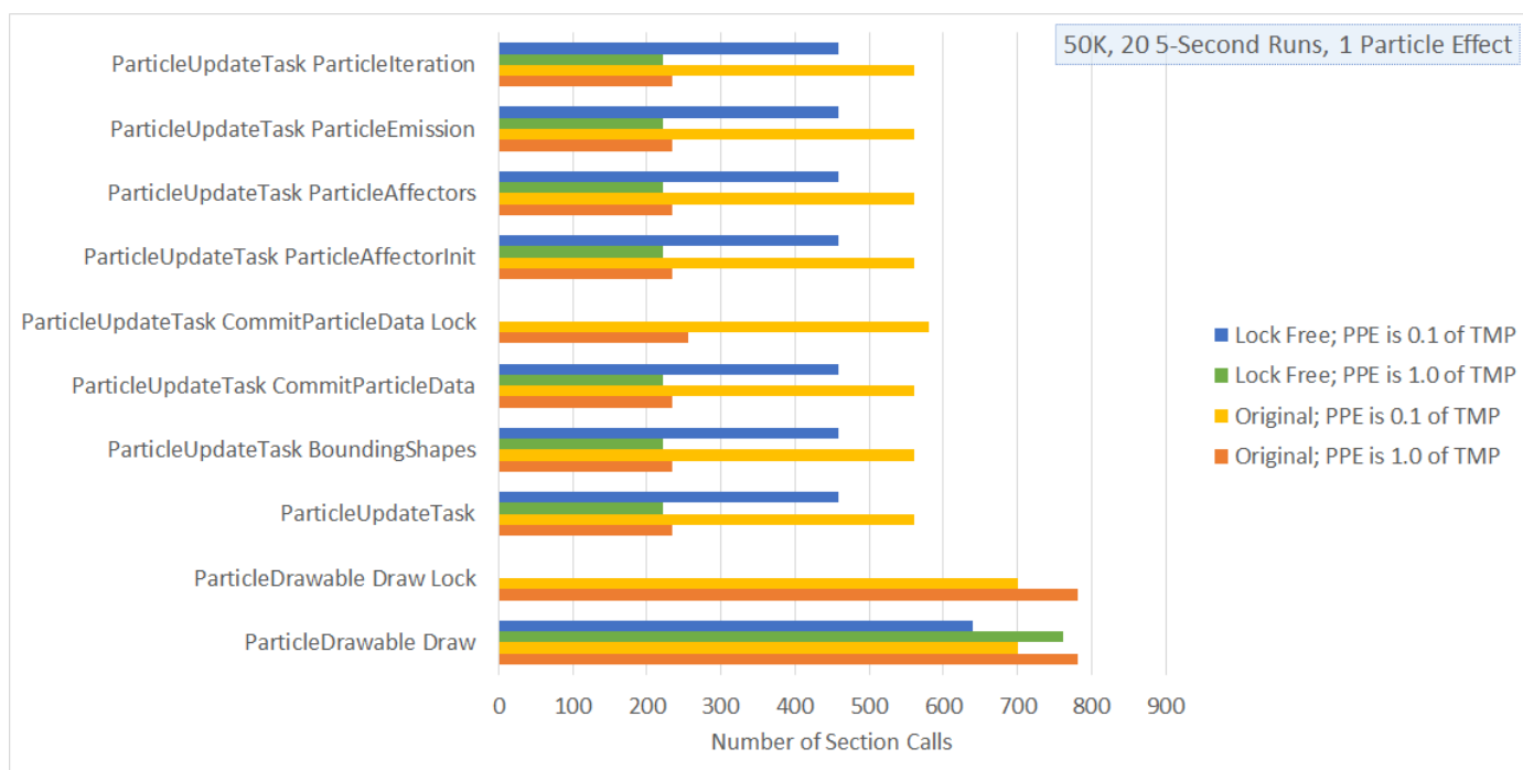
Figure 5.8 A graph showing the number of section calls for various sections of code for a single particle effect.
