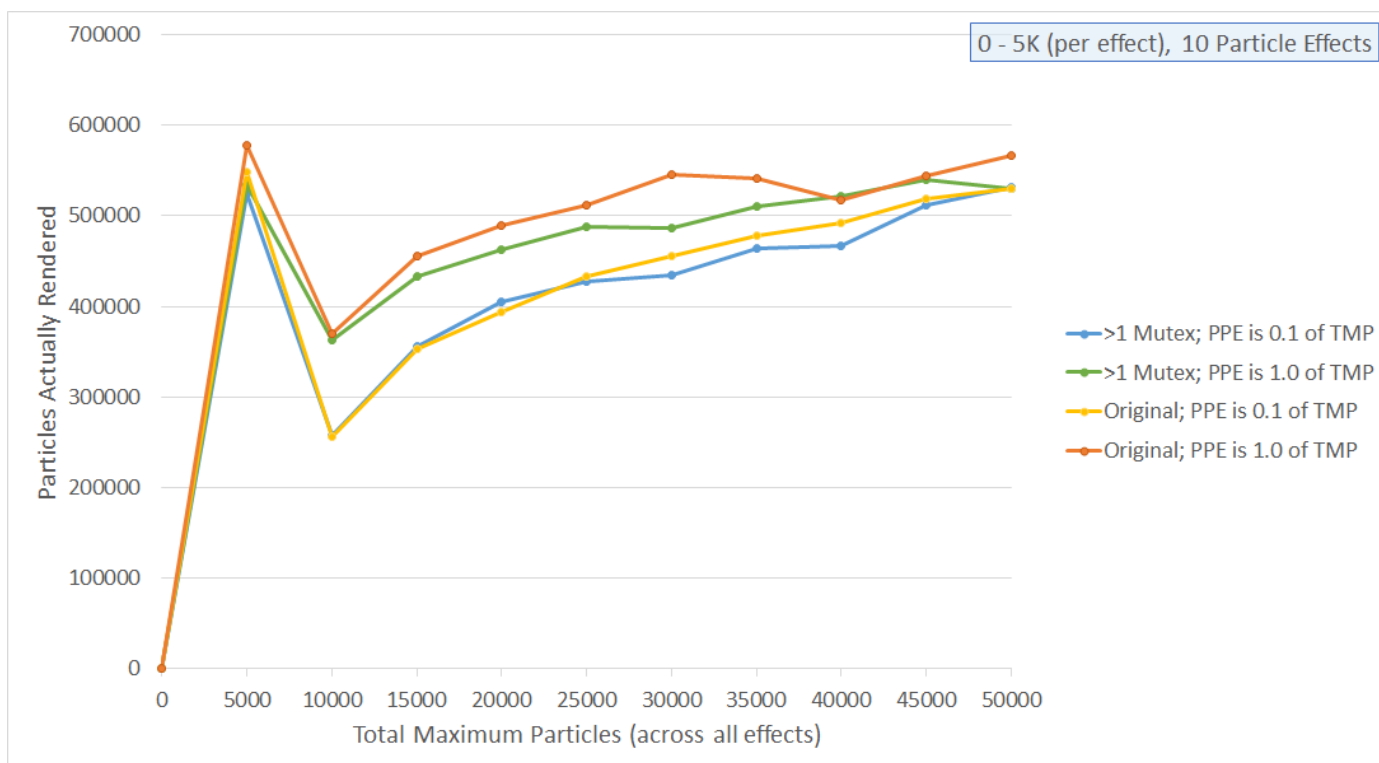
Figure 5.11 A graph showing particles actually rendered over total maximum particles for ten particle effects.
