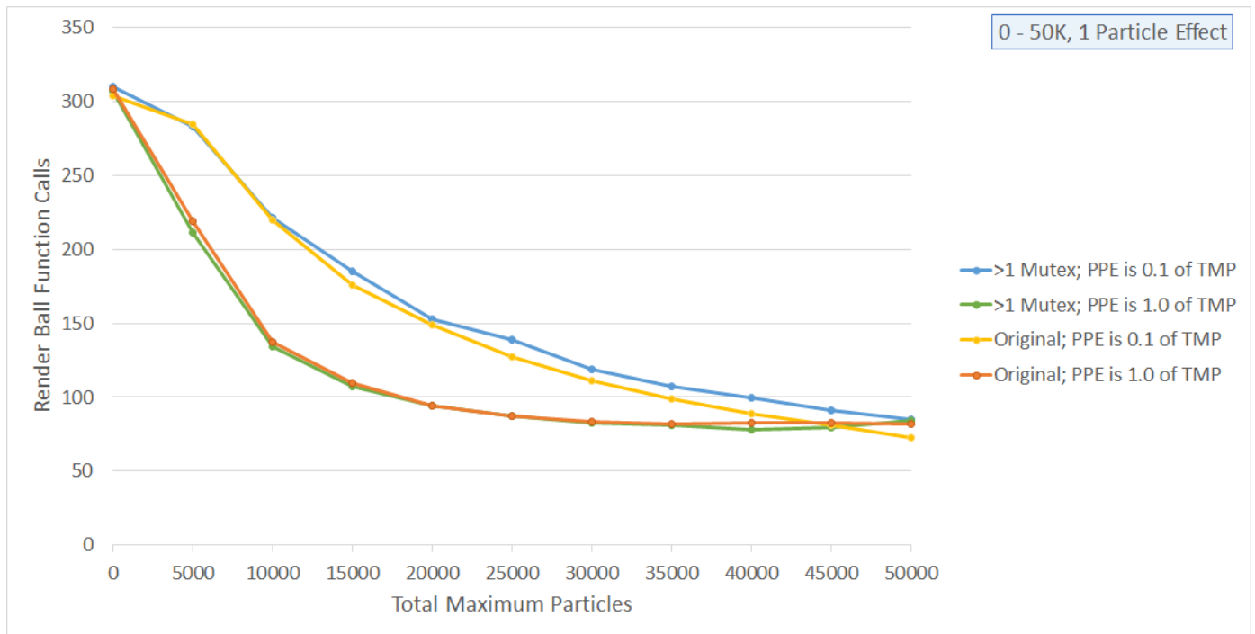
Figure 5.2 A graph showing render ball function calls over total maximum particles for a single particle effect.
