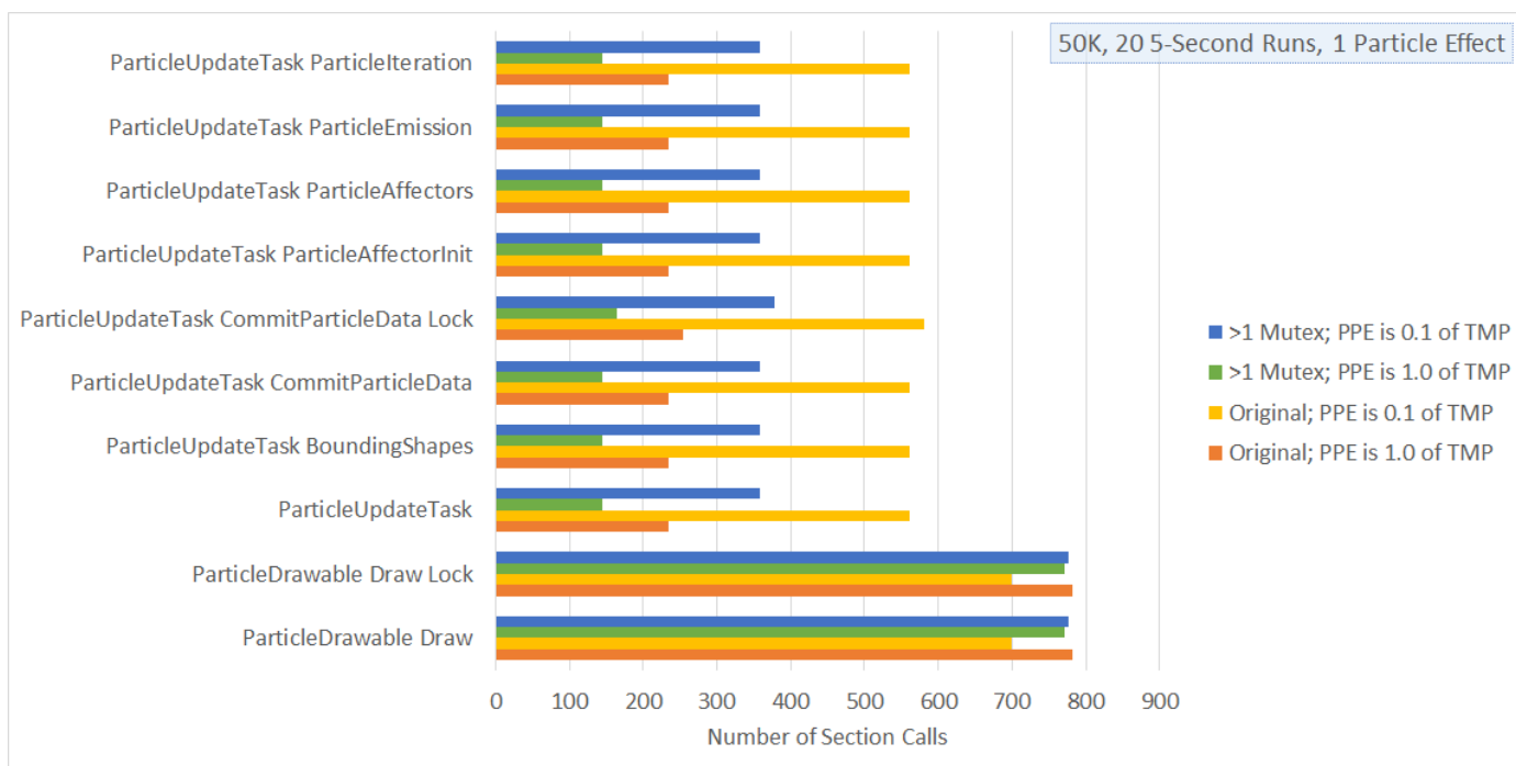
Figure 5.4 A graph showing the number of section calls for various sections of code for a single particle effect. Note that the "ParticleUpdateTask CommitParticleData Lock" section is timing the particle array lock for the "> 1 Mutex" data series.
