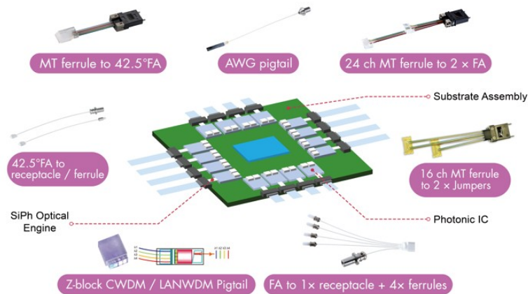
Exhibit 5: FOCI's solutions for CPO
