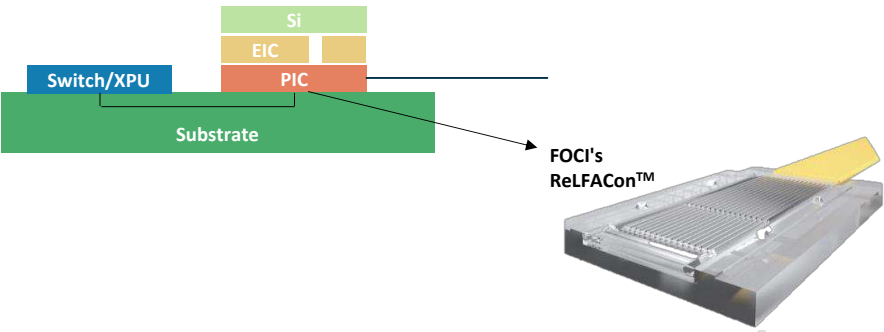
Exhibit 6: ReLFACon enables direct transmission of external photonic signals with MCM modules to achieve reliable signal transmission
