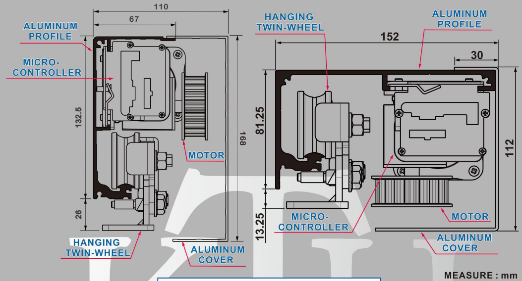
MICRO-CONTROLLER COMBINED TERMINAL BLOCK K-2(EN-16005)
