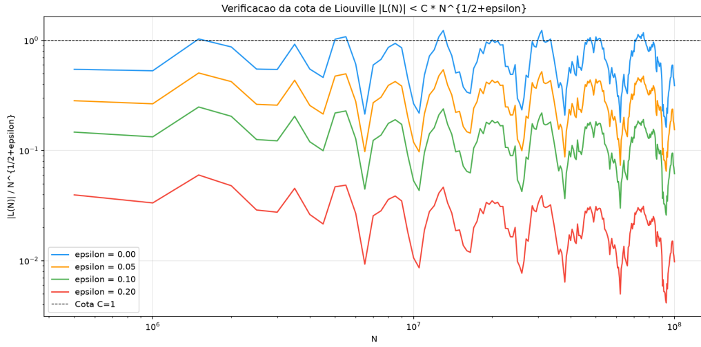
Figure 2: Razão |L(N)|/N^{1/2+\varepsilon} para \varepsilon = 0, 0.05, 0.10, 0.20 .
