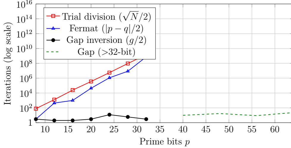
Figure 5: Scaling of methods: trial division and Fermat grow exponentially with bit size; gap inversion remains \mathcal{O}(1) .
