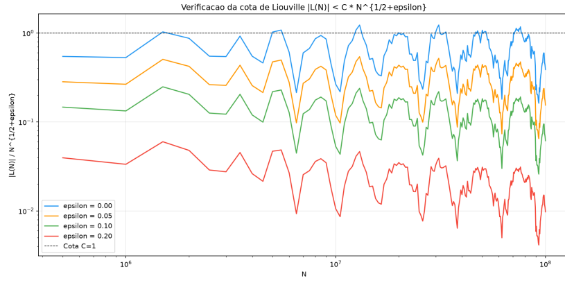
Figure 2: Ratio |L(N)|/N^{1/2+\varepsilon} for \varepsilon = 0, 0.05, 0.10, 0.20 .
