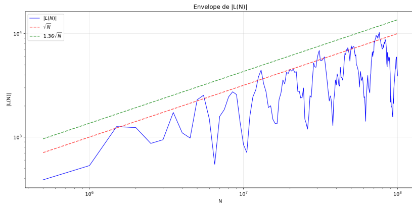
Figure 3: |L(N)| vs. \sqrt{N} and 1.36\sqrt{N} .
