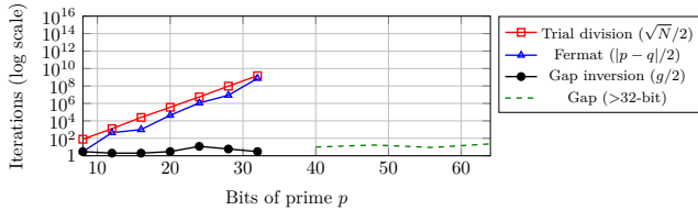
Figure 6. Scaling of methods: trial division and Fermat grow exponentially with bit size; gap inversion remains \mathcal{O}(1) .
