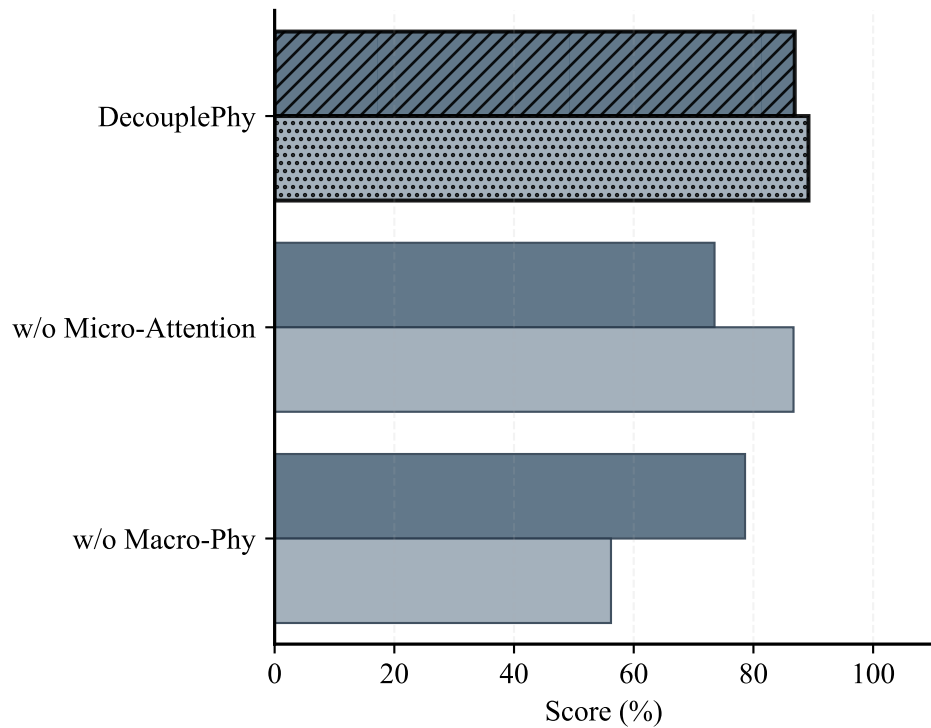
Ablation: BATADAL
