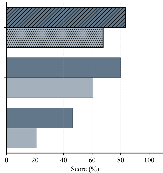
Ablation: SWaT
