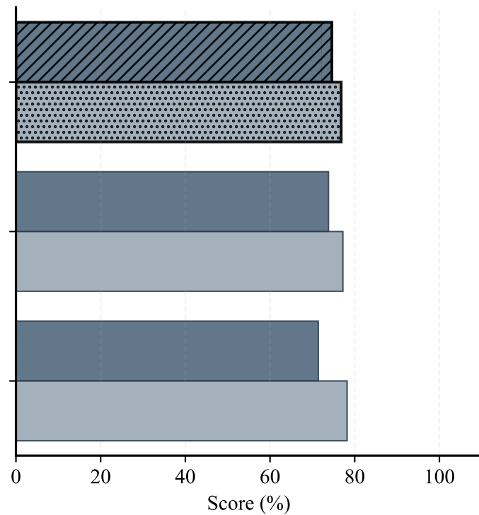
Ablation: HAI
