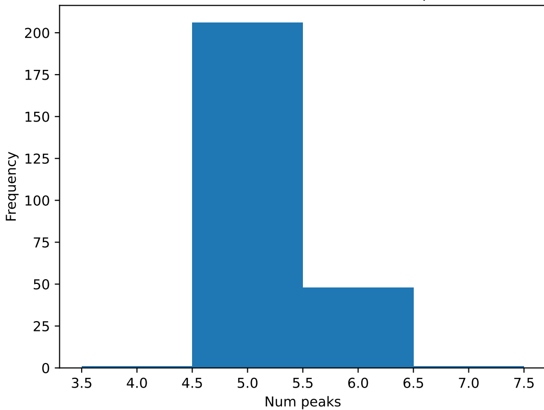
Posterior distribution of number of peaks
