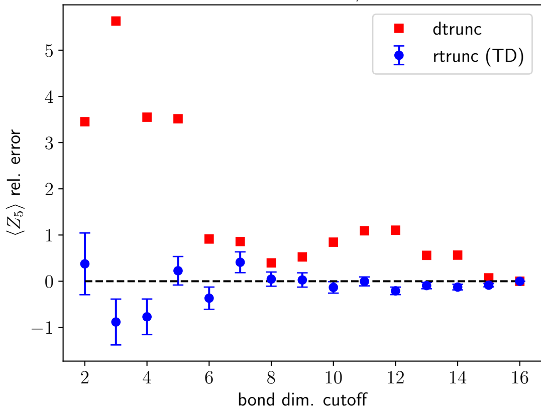
MPS on 9 sites, \gamma=0.2
