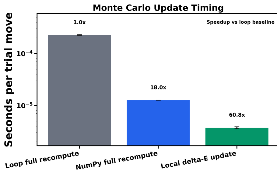
Fig. S3 The local \Delta E benchmark separates algorithmic improvement from NumPy vectorisation. Avoiding whole-lattice recomputation gives the largest speedup.
