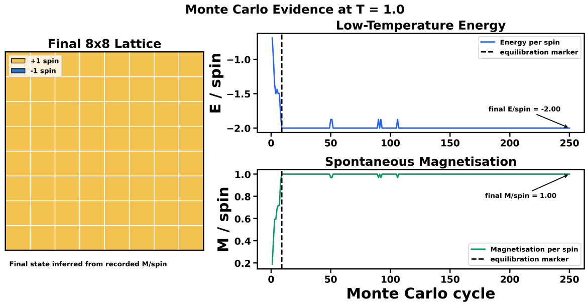
Fig. S2 The 8 \times 8 lattice reaches the fully ordered state at T = 1.0 . The trajectory provides a low-temperature ordering check, not a guarantee of rapid equilibration near T_C .
