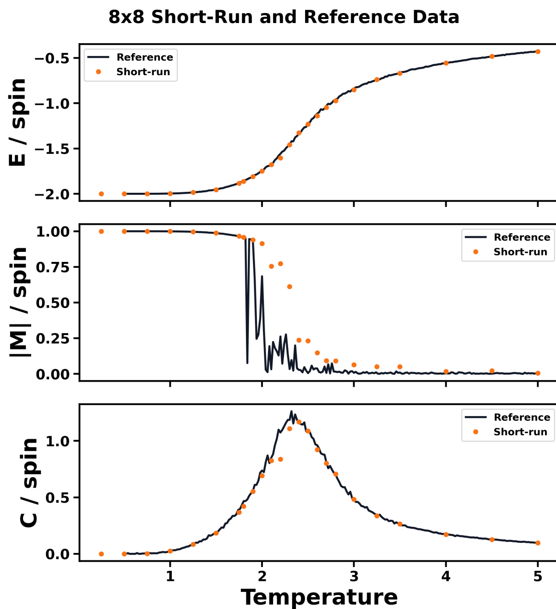
Fig. S11 Short-run and reference 8 \times 8 data agree in the main thermodynamic trends. The short-run simulation data are visibly noisier near the heat-capacity peak.
