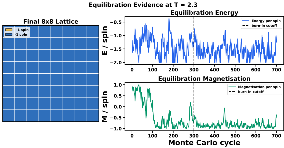
Fig. S4 The 300-cycle burn-in cut removes the main relaxation transient from the 8 \times 8 production statistics near T = 2.3 .
