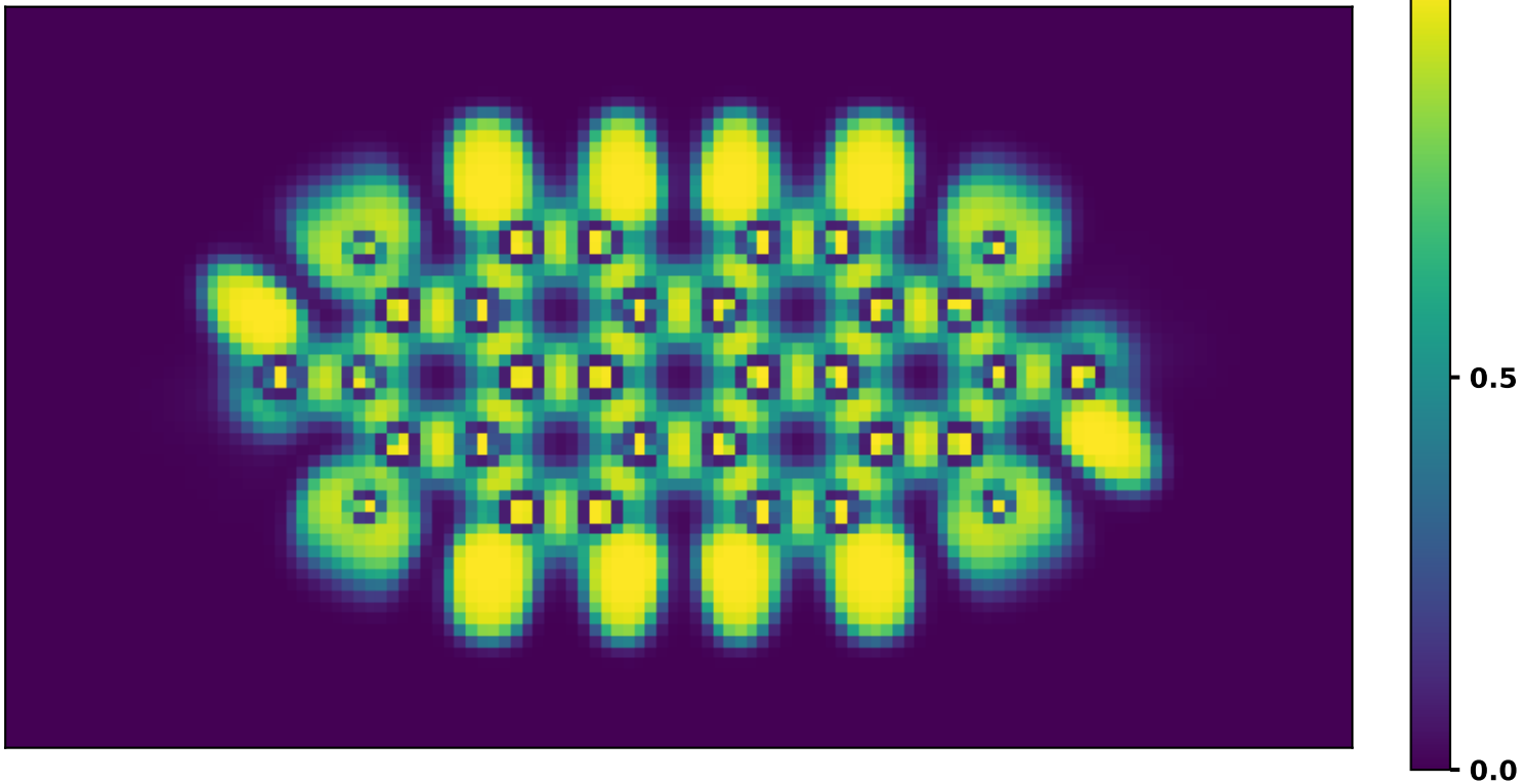
Terminal-functionalized PDI, ELF central slice
