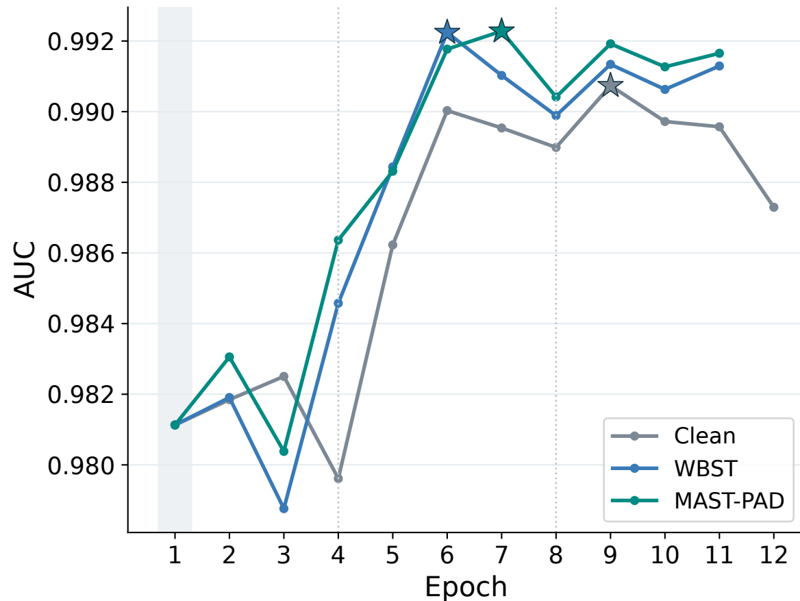
A Source-selection AUC
