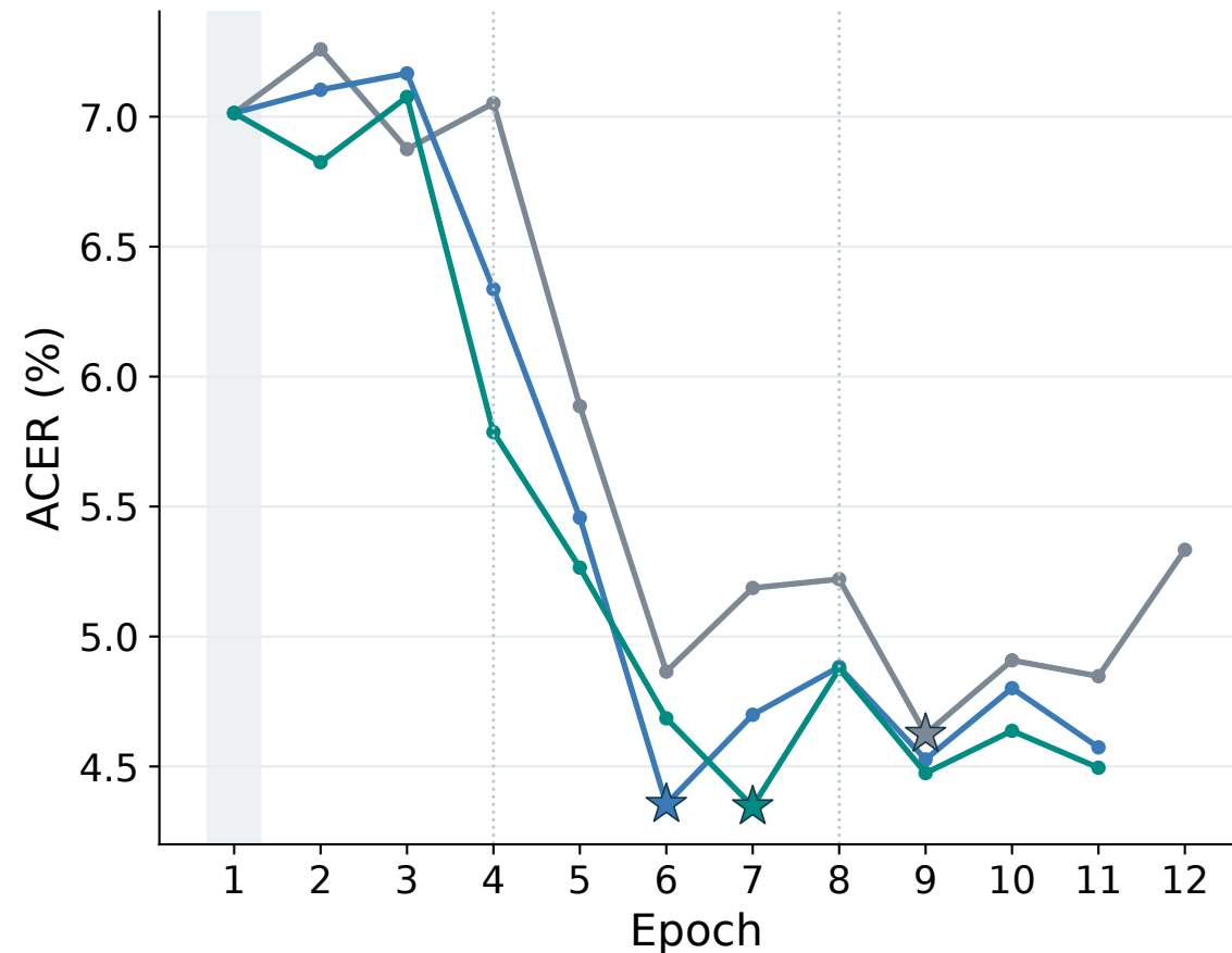
B Source-selection ACER
