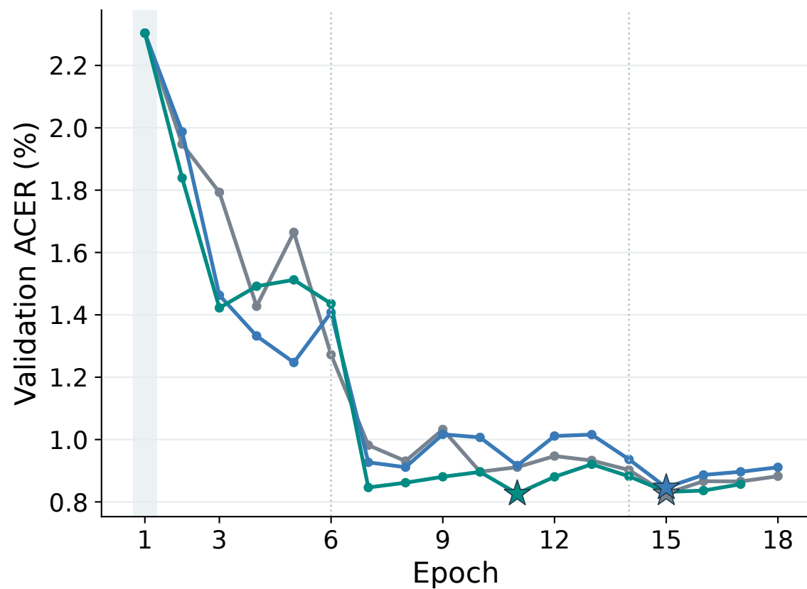
B Validation ACER
