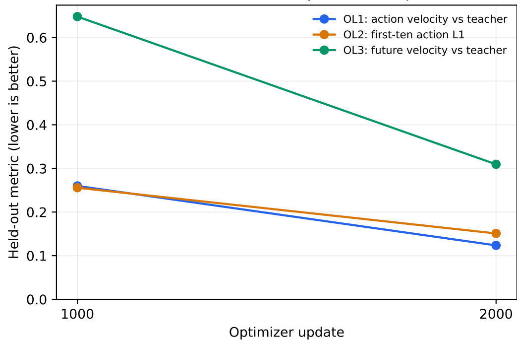
EMA on the fixed 20-clip validation panel
