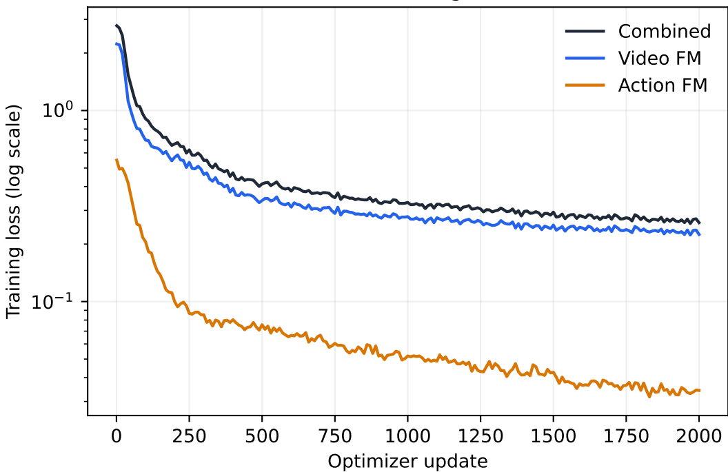
Phase 0: fixed (4,4), L2, global batch 128
