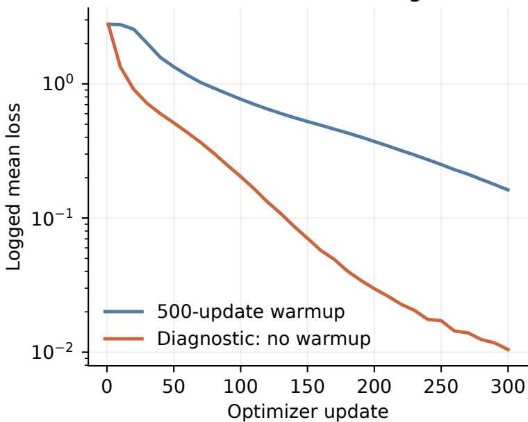
Combined flow-matching loss
