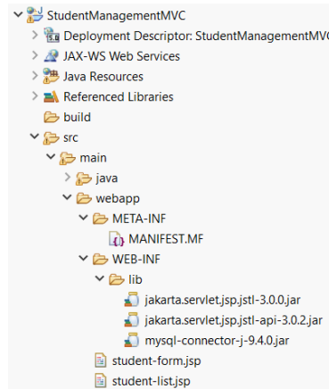
Project Structure
