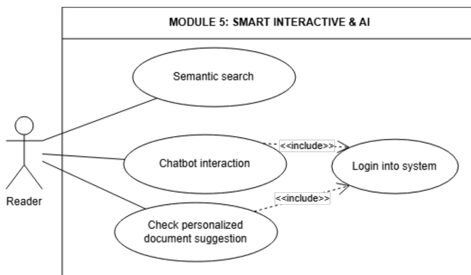
Figure 10: Intelligent Interaction & AI Use-Case Diagram
