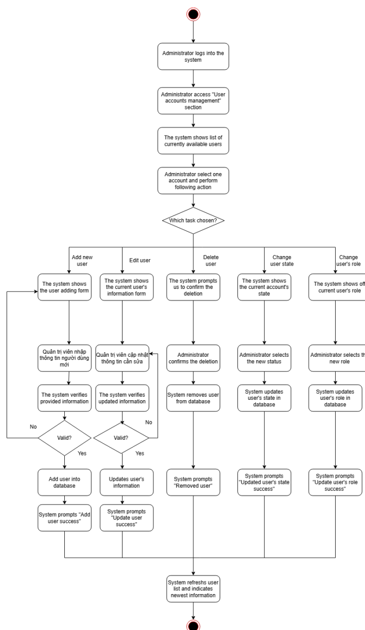
Figure 27: Activity Diagram for User Account Management
