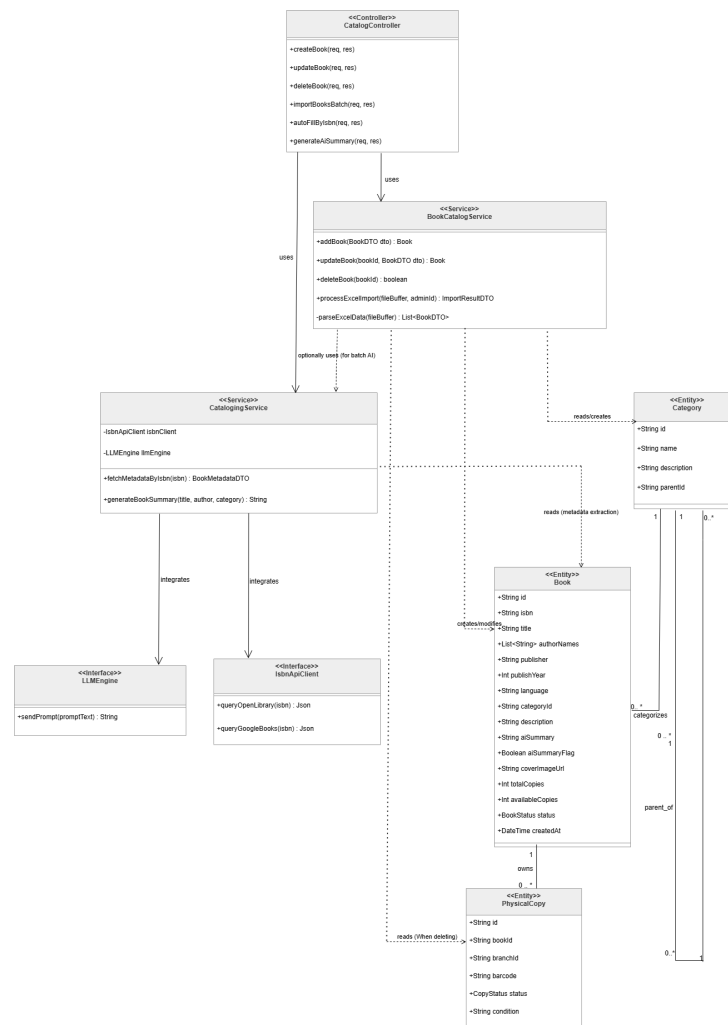
Figure 17: Class Diagram for Book Catalog Management
