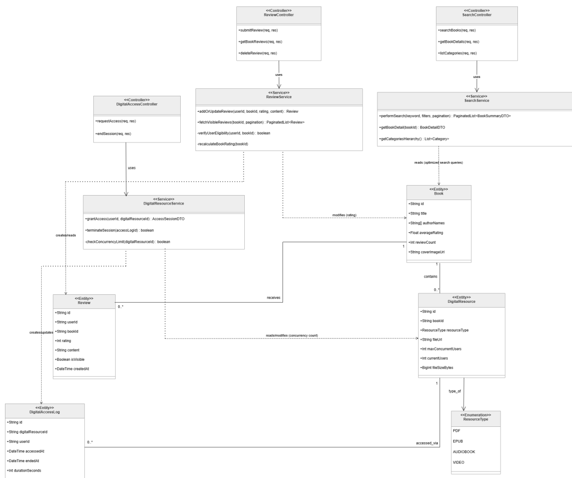
Figure 19: Class Diagram for Resource Search and Exploitation
