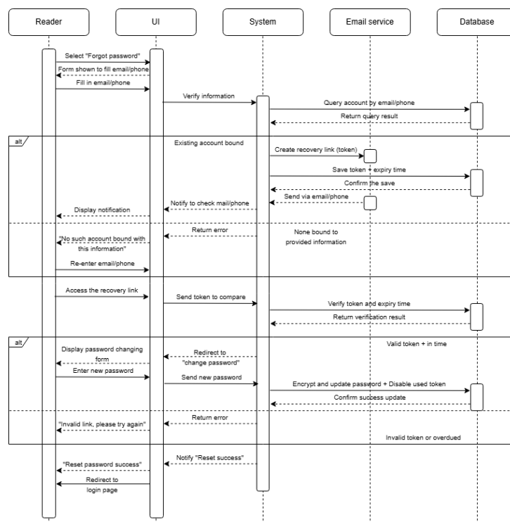
Figure 39: Sequence Diagram for Account Password Reset
