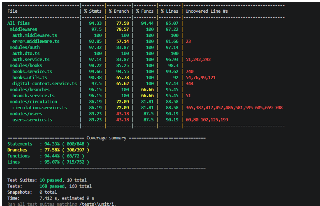
Figure 80: Unit test results
