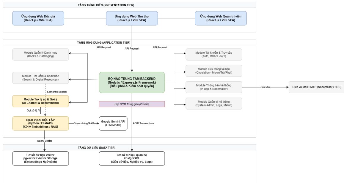
Figure 13: Overall System Architecture Diagram of the Online Library Management System
