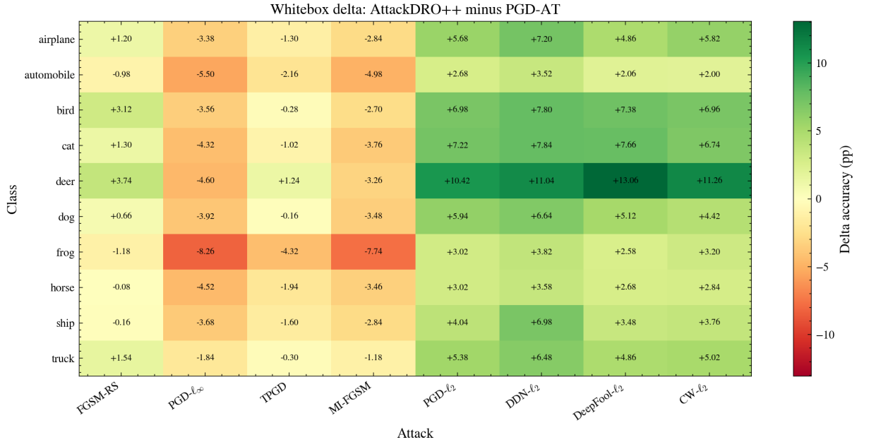
Figure 6.7: Whitebox per-(class \times attack) delta of AttackDRO++ (Ours) relative to PGD-AT, averaged over five seeds. Cells report AttackDRO++ minus PGD-AT in percentage points; positive values indicate where AttackDRO++ (Ours) improves over the PGD- \ell_\infty specialist.
