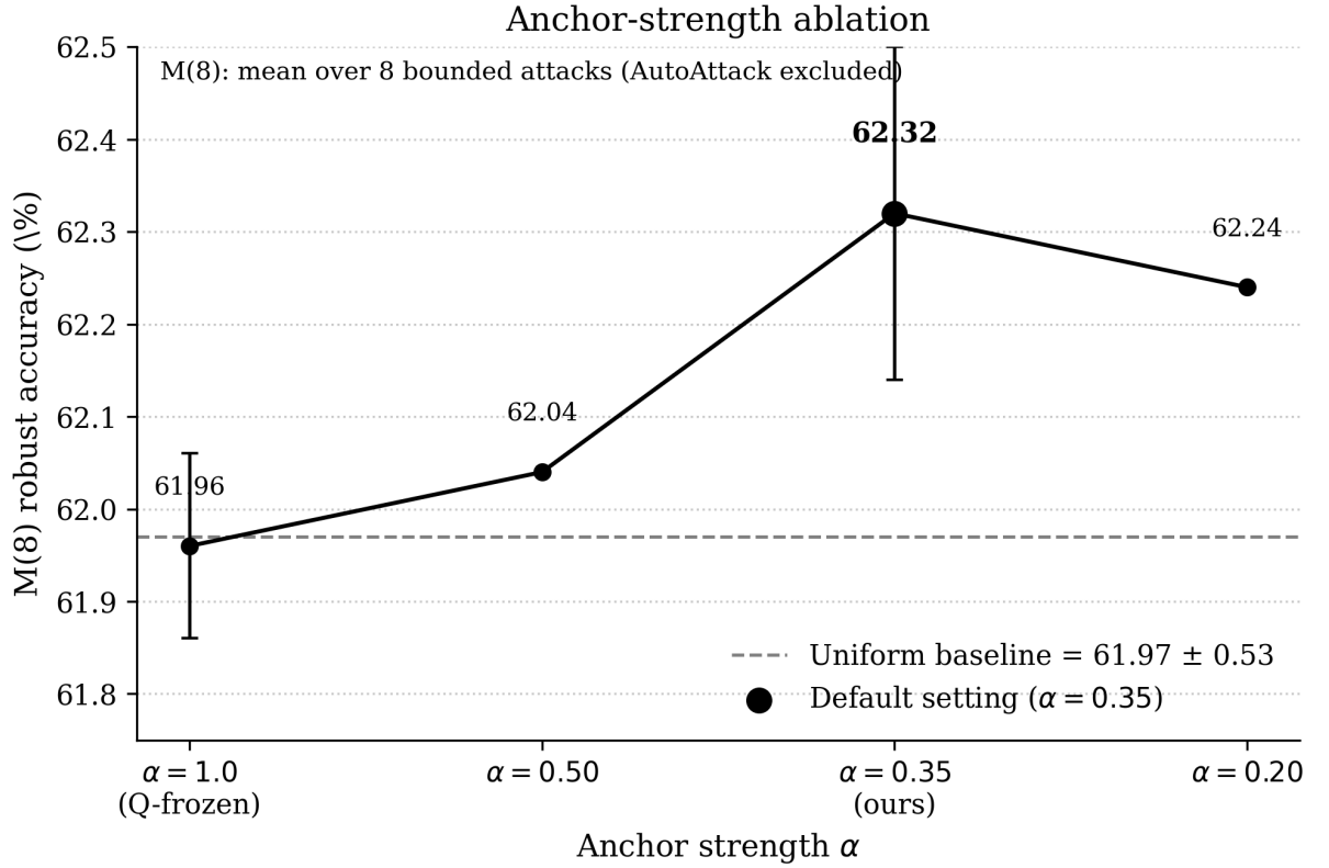
Figure 6.22: Ablation dashboard for AttackDRO++. The dashboard summarizes the sensitivity of M(8) robust accuracy to anchor strength, number of clusters, and cluster-refresh schedule. M(8) denotes the mean robust accuracy over the eight bounded evaluation attacks and excludes AutoAttack.
