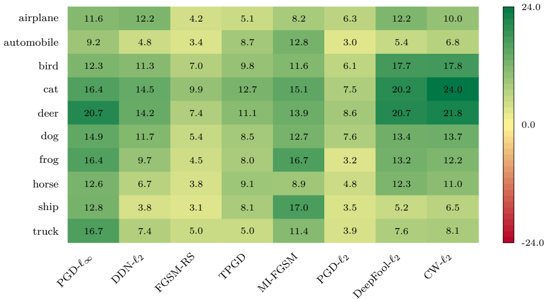
graybox - whitebox gap: AttackDRO++
