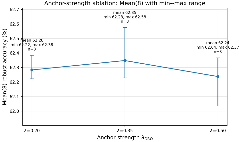
Figure 6.23: Sensitivity of AttackDRO++ to the anchor strength \lambda_{\text{DRO}} . The figure reports Mean(8) robust accuracy with the min–max range across available runs. Mean(8) is computed over the eight non-AutoAttack evaluation attacks. The previous \lambda_{\text{DRO}} = 1.0 setting is excluded from the final ablation panel.
