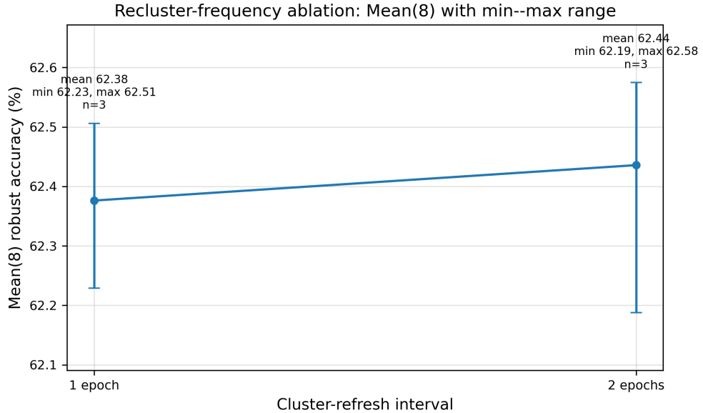
Figure 6.24: Sensitivity of AttackDRO++ to the cluster-refresh interval. The figure reports Mean(8) robust accuracy with the min–max range across available runs. Mean(8) is computed over the eight non-AutoAttack evaluation attacks. The two refresh schedules produce similar results, so the default two-epoch schedule is retained as a practical stability choice.
