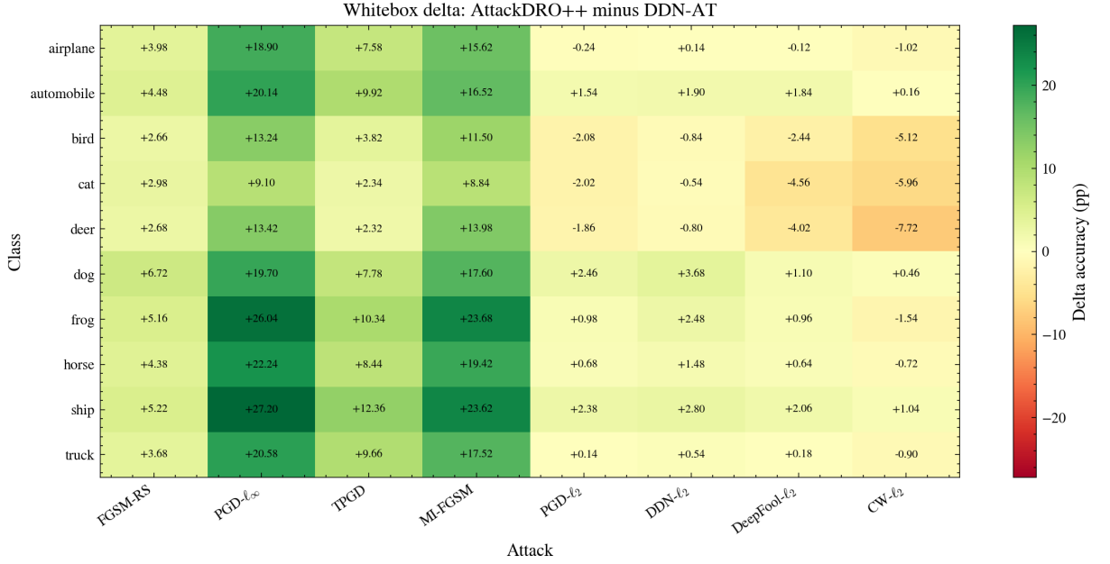
Figure 6.8: Whitebox per-(class \times attack) delta of AttackDRO++ (Ours) relative to DDN-AT, averaged over five seeds. Cells report AttackDRO++ minus DDN-AT in percentage points; positive values indicate where AttackDRO++ (Ours) improves over the DDN- \ell_2 specialist.
