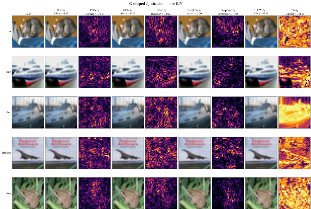
Figure C.2: Grouped \ell_2 adversarial examples on CIFAR-10, with adversarial images and normalized perturbation heatmaps.
