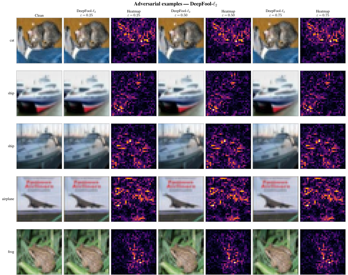
Figure 2.6: DeepFool- \ell_2 adversarial examples on CIFAR-10 under three perturbation budgets, with normalized boundary-oriented perturbation heatmaps.
