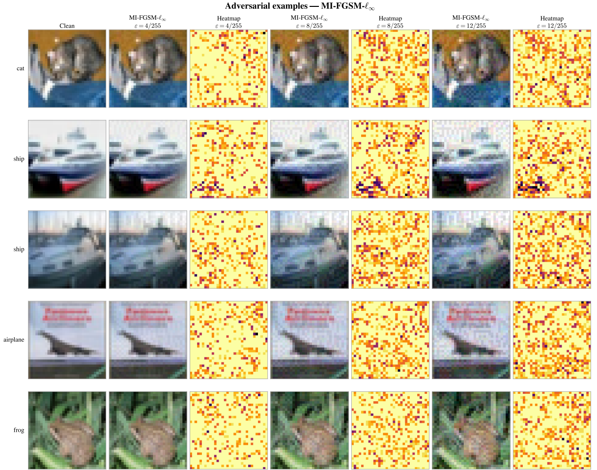
Figure 2.8: MI-FGSM- \ell_\infty adversarial examples on CIFAR-10 under three perturbation budgets, with normalized perturbation heatmaps.
