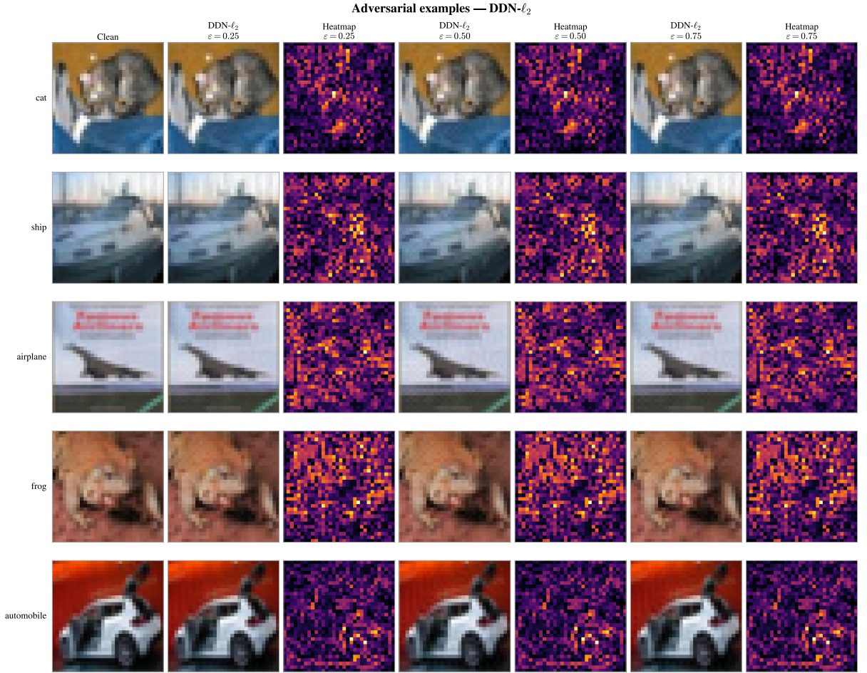
Figure 2.7: DDN- \ell_2 adversarial examples on CIFAR-10 under three perturbation budgets, with normalized perturbation heatmaps.
