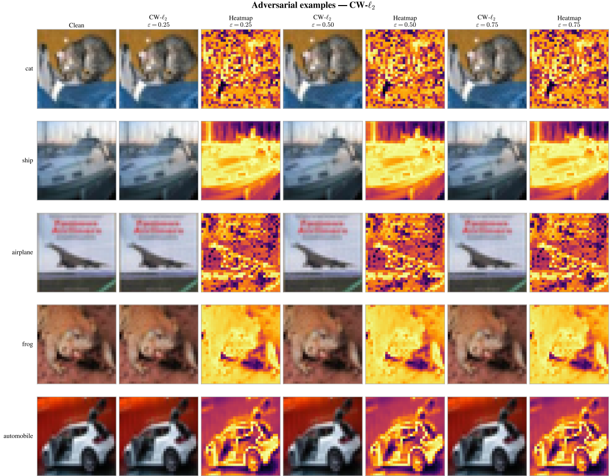
Figure 2.5: CW- \ell_2 adversarial examples on CIFAR-10 under three perturbation budgets, with normalized perturbation heatmaps.
