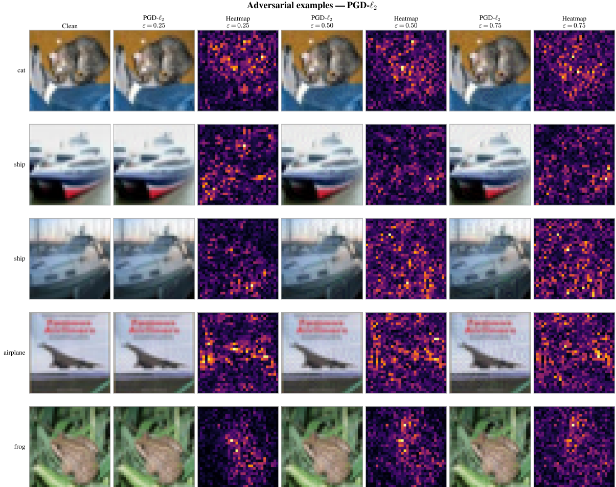
Figure 2.4: PGD- \ell_2 adversarial examples on CIFAR-10 under three perturbation budgets, with normalized perturbation heatmaps.
