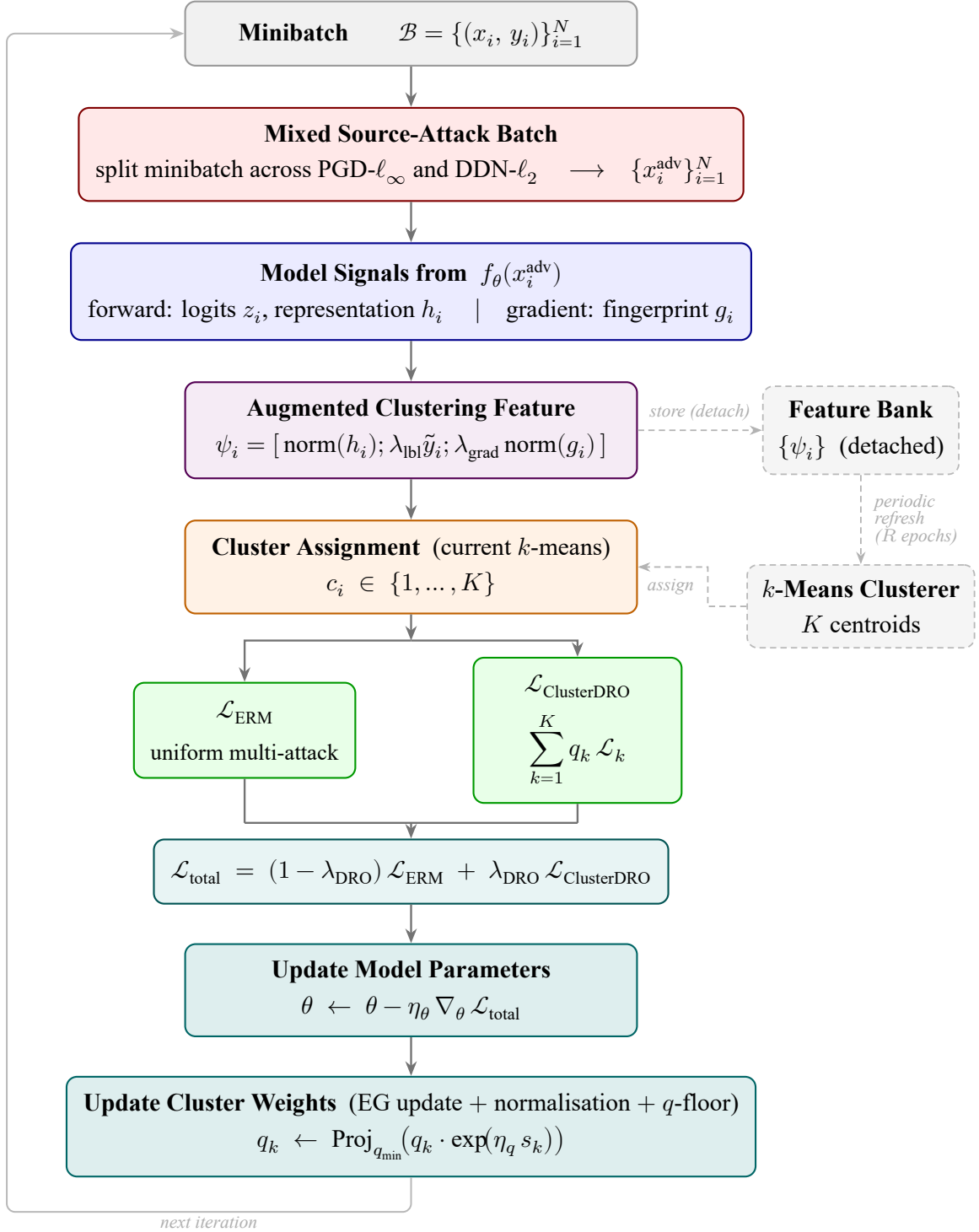
Figure 4.2: Core training loop of AttackDRO++. A minibatch is converted into a mixed PGD- \ell_\infty /DDN- \ell_2 adversarial batch, passed through the model to construct augmented clustering features \psi_i , assigned to latent clusters, and optimized with a uniform-anchored combination of ERM and Cluster-DRO losses. Cluster weights \mathbf{q} and K-means centroids are updated periodically according to the configured refresh and reweighting policy.
