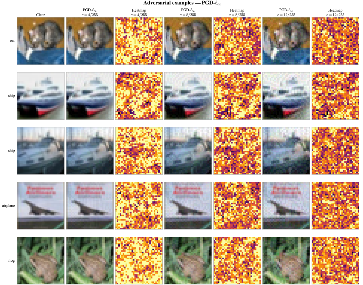
Figure 2.3: PGD- \ell_\infty adversarial examples on CIFAR-10 under three perturbation budgets, with normalized perturbation heatmaps.
