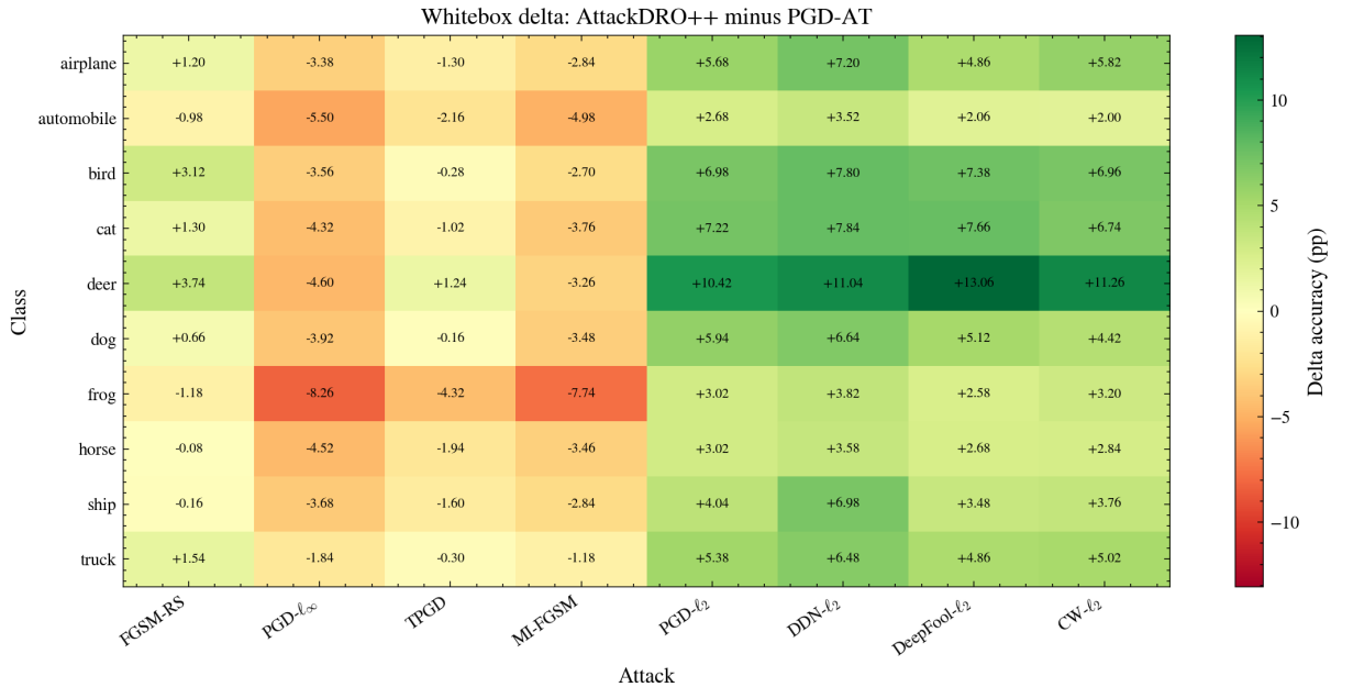
Figure 6.7: Whitebox per-(class \times attack) delta of AttackDRO++ relative to PGD-AT, averaged over five seeds. Cells report AttackDRO++ minus PGD-AT in percentage points; positive values indicate where AttackDRO++ improves over the PGD- \ell_\infty specialist.
