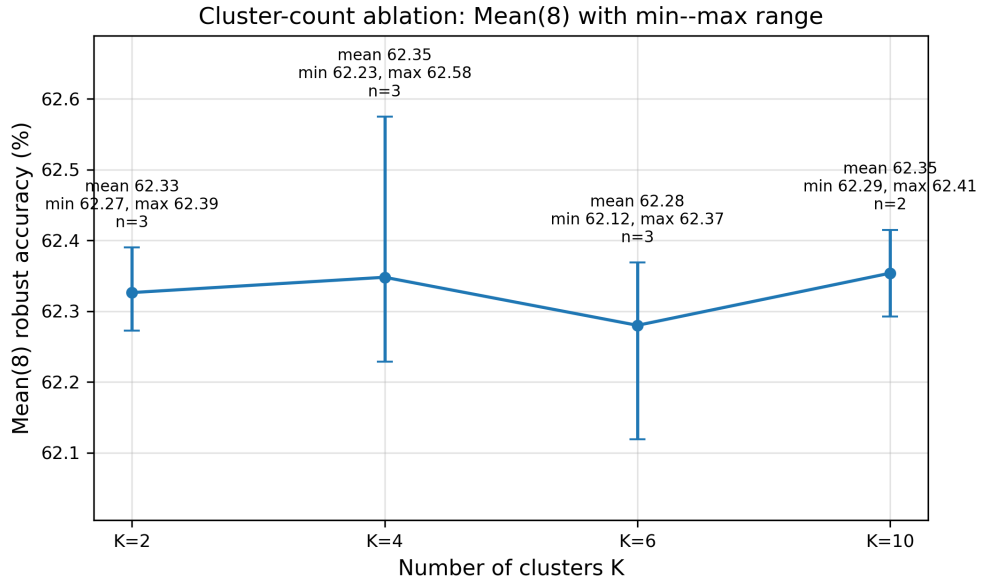
Figure 6.22: Sensitivity of AttackDRO++ to the number of clusters. Points show Mean(8) robust accuracy with the min-to-max range across available runs; Mean(8) is computed over the eight non-AutoAttack evaluation attacks.
