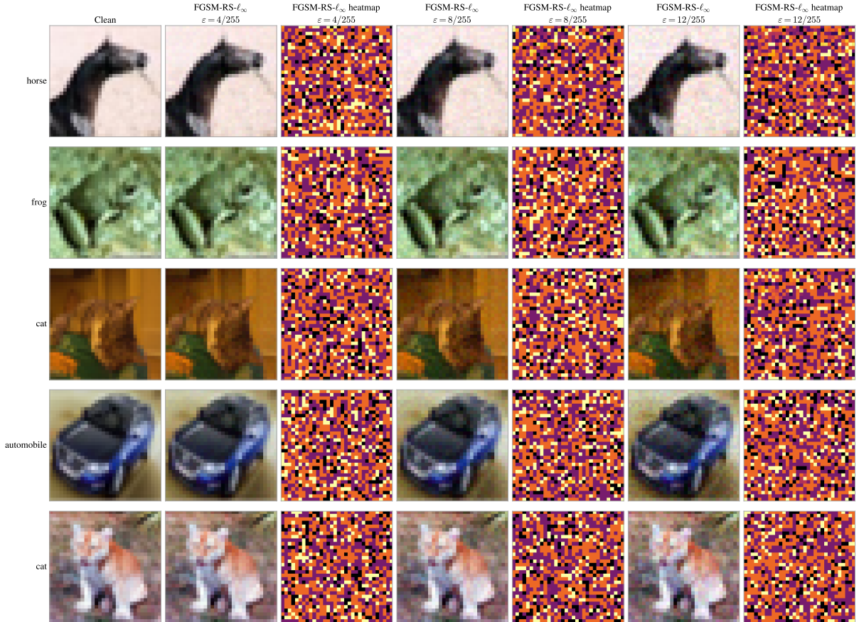
Figure 2.1: FGSM-RS- \ell_\infty adversarial examples on CIFAR-10 under three perturbation budgets. Each row shows the clean image, adversarial image, and normalized perturbation heatmap.
