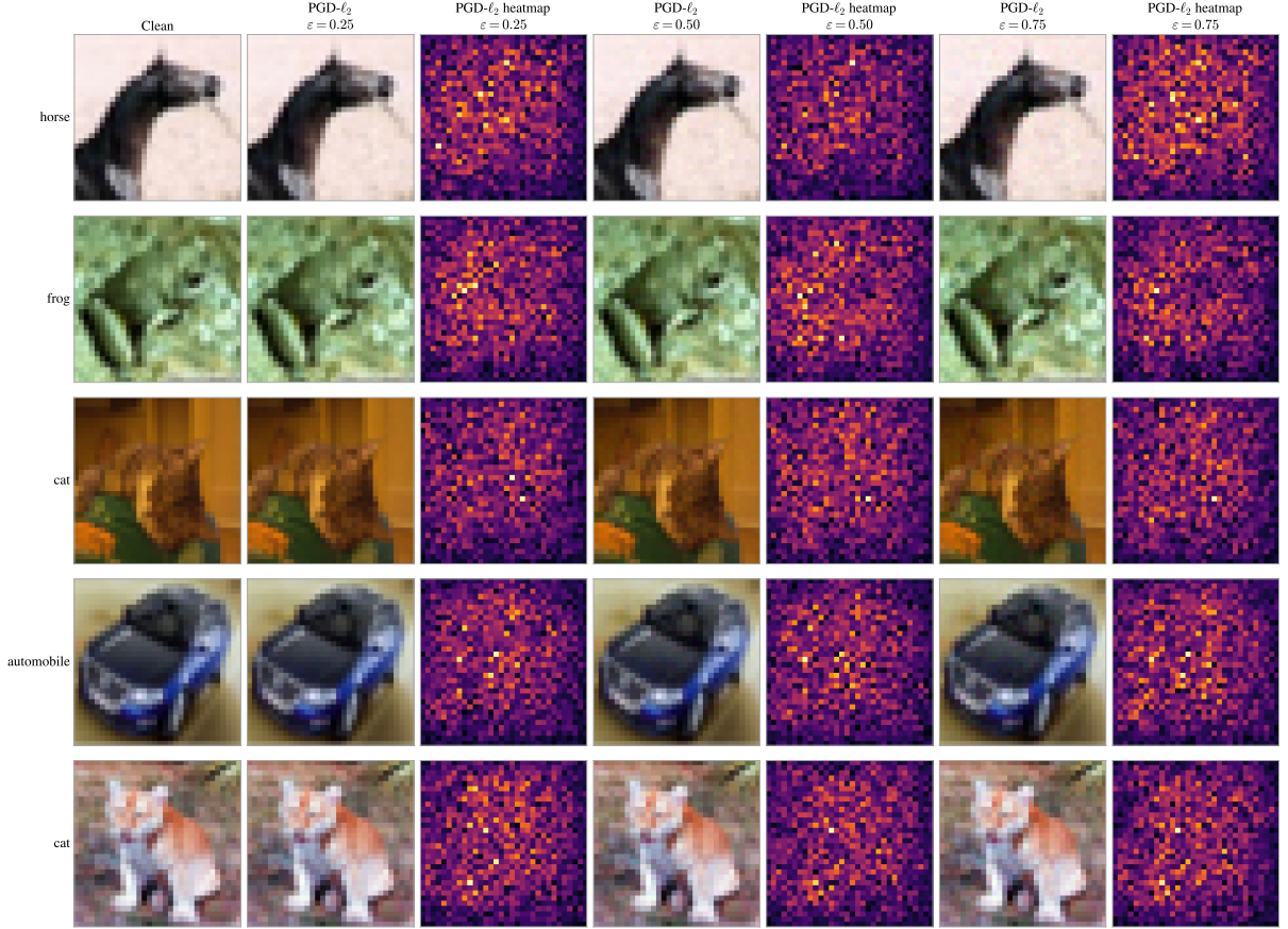
Figure 2.3: PGD- \ell_2 adversarial examples on CIFAR-10 under three perturbation budgets, with normalized perturbation heatmaps.
