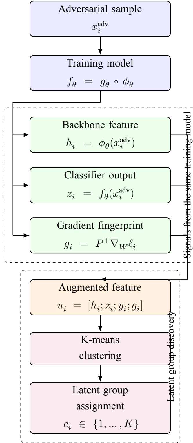
Figure 4.1: Augmented clustering feature construction in AttackDRO++. Each adversarial sample x_i^{\text{adv}} is passed through the same training model f_\theta , producing both the backbone feature h_i and classifier output z_i . A gradient fingerprint g_i is computed from the classifier-head loss gradient and projected to a low-dimensional vector. The feature, prediction signal, label information, and gradient fingerprint are combined as u_i = [h_i; z_i; y_i; g_i] , which is then used for K-means clustering and latent group assignment.
