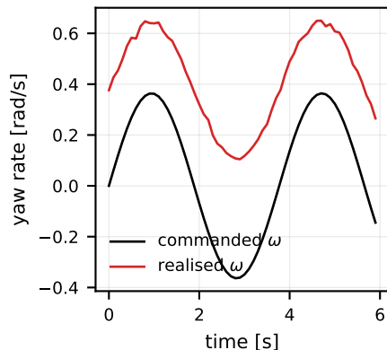
gain-L fault: command vs realised
