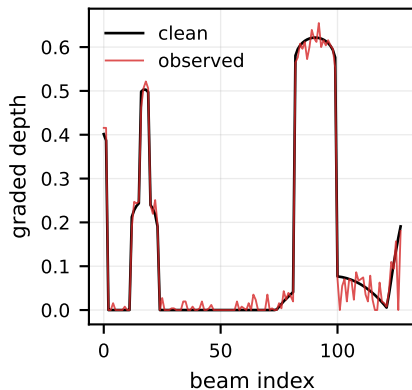
depth profile (120°, 128 beams)
